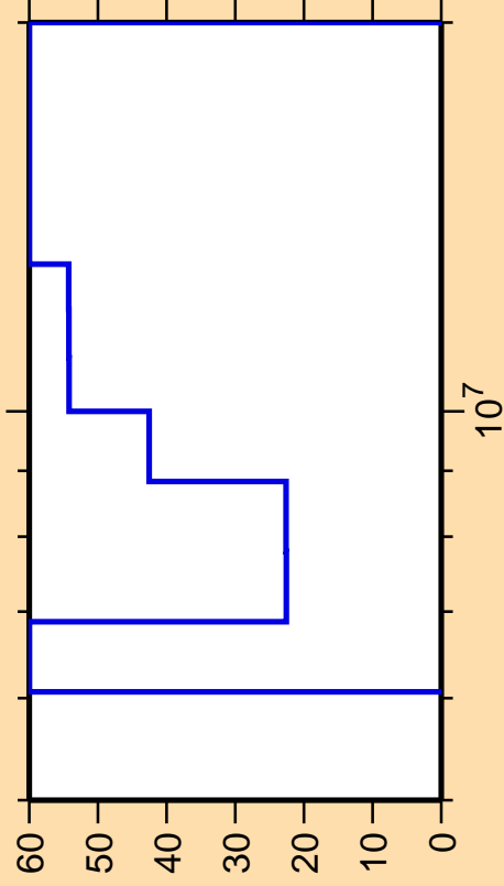
\Delta\sigma/\sigma vs. E for ^{232}\text{Np}(n,\gamma)
