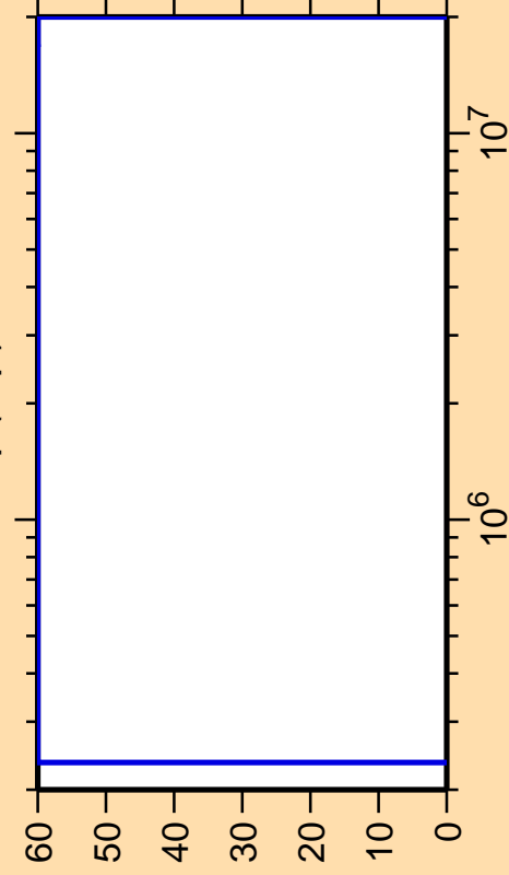
\Delta\sigma/\sigma vs. E for ^{232}\text{Np}(n,p)
