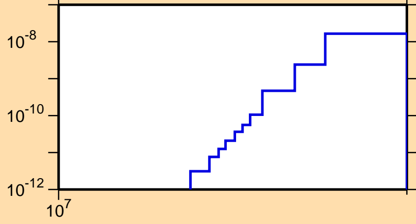
\sigma vs. E for ^{232}\text{Np}(n,\text{He3})
