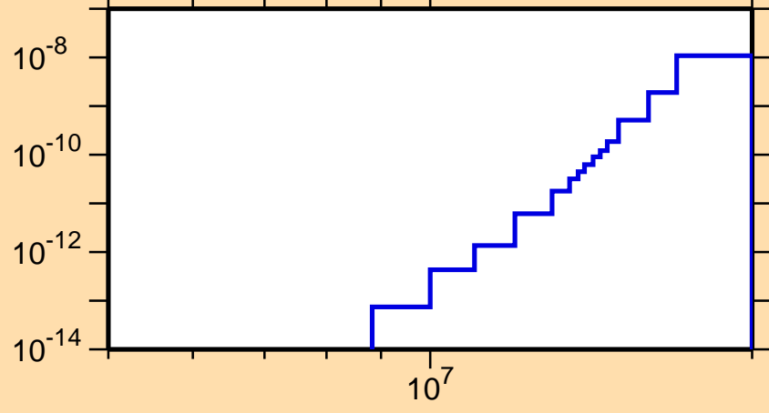
\sigma vs. E for ^{232}\text{Np}(n,2n\alpha)
