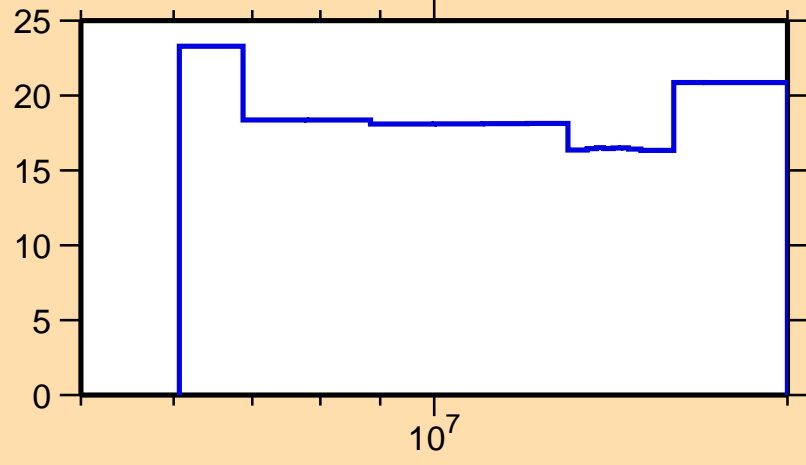
\Delta\sigma/\sigma vs. E for ^{232}\text{Np}(n,\text{inel.})
