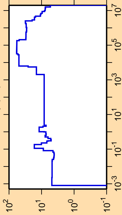
\Delta\sigma/\sigma vs. E for ^{232}\text{Np}(n,f)
