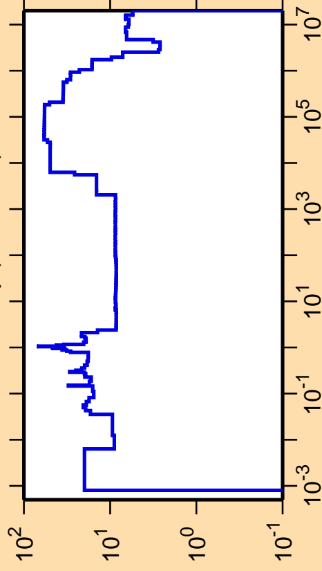
\Delta\sigma/\sigma vs. E for ^{232}\text{Np}(n,\text{nonel.})
