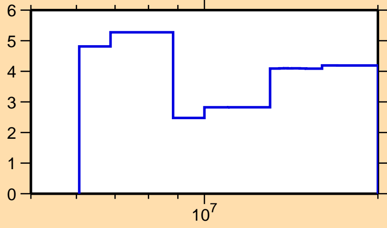
\Delta\sigma/\sigma vs. E for ^{232}\text{Np}(n,\text{tot.})
