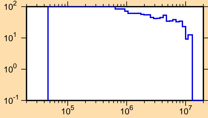
\Delta\sigma/\sigma vs. E for ^{232}\text{Np}(n,n_1)
