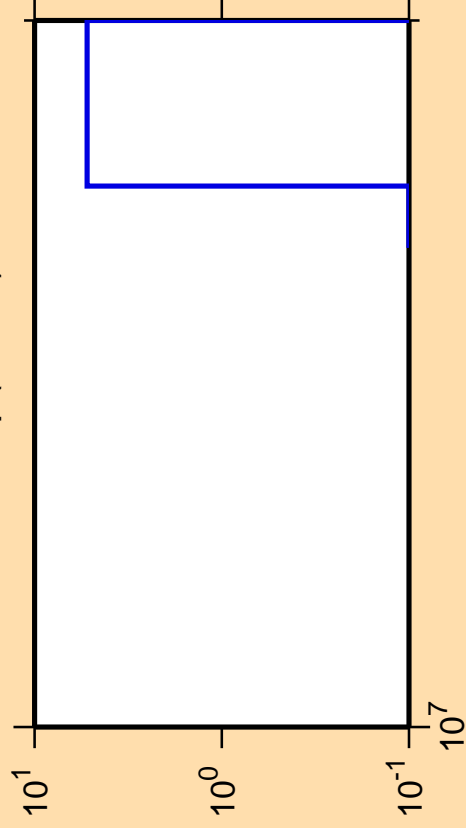
\Delta\sigma/\sigma vs. E for ^{232}\text{Np} (mt 34)
