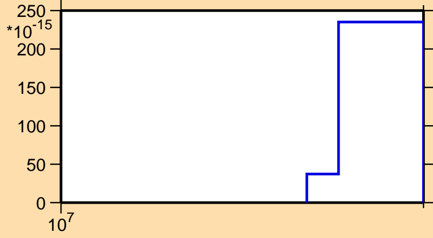
\sigma vs. E for ^{232}\text{Np} (mt 45)
