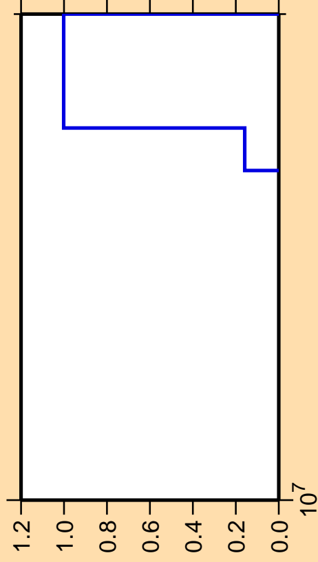
\Delta\sigma/\sigma vs. E for ^{232}\text{Np} (mt 45)
