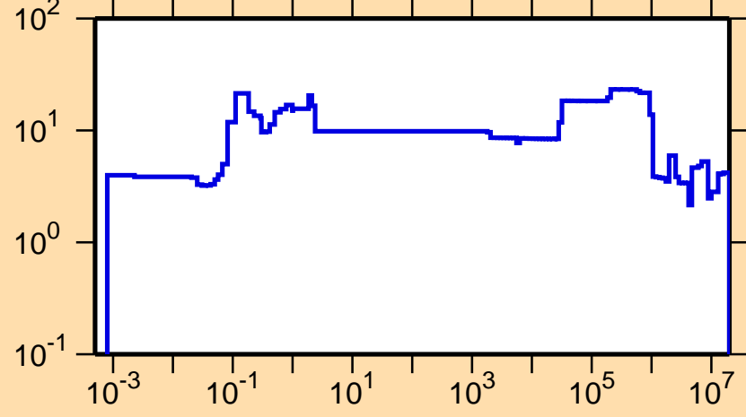
\Delta\sigma/\sigma vs. E for ^{232}\text{Np}(n,tot.)
