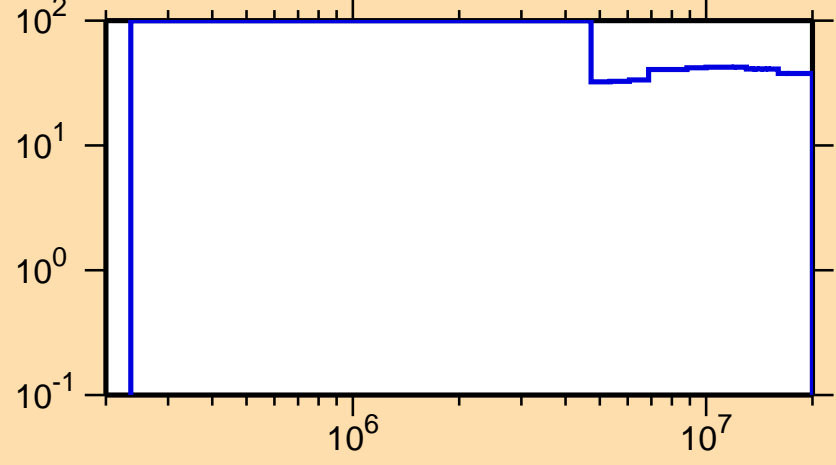
\Delta\sigma/\sigma vs. E for ^{232}\text{Np}(n,ncont.)
