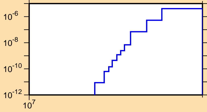
\sigma vs. E for ^{232}\text{Np}(n,2np)
