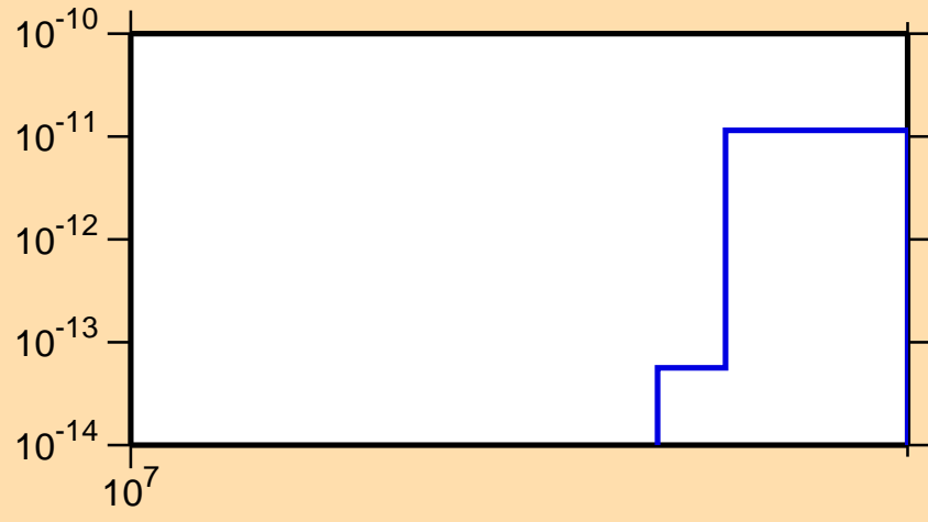
\sigma vs. E for ^{232}\text{Np}(n,3n\alpha)
