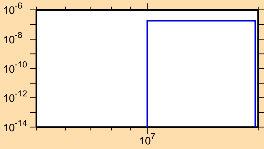
\sigma vs. E for ^{232}\text{Np}(n,\text{nd})
