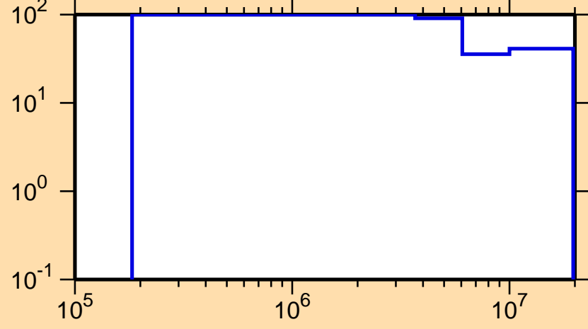
\Delta\sigma/\sigma vs. E for ^{232}\text{Np}(n,n\text{cont.})
