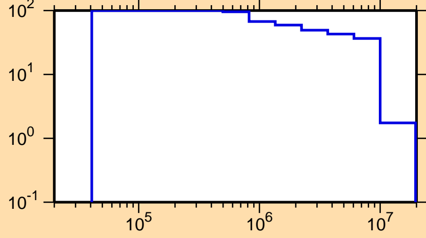
\Delta\sigma/\sigma vs. E for ^{232}\text{Np}(n,n_1)
