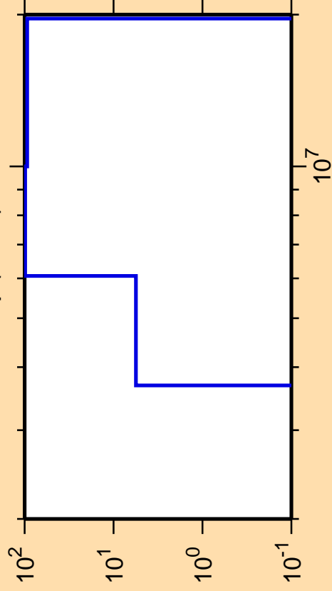
\Delta\sigma/\sigma vs. E for ^{232}\text{Np}(n,n\alpha)
