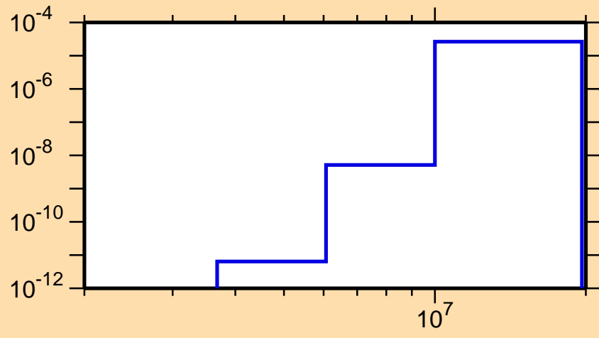
\sigma vs. E for ^{232}\text{Np}(n,n\alpha)
