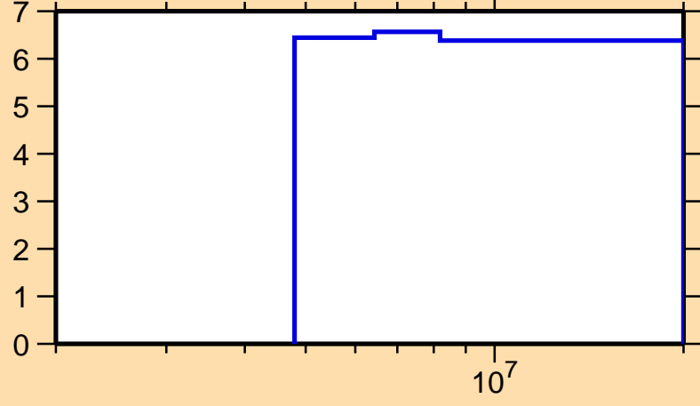
\Delta\sigma/\sigma vs. E for ^{232}\text{Np}(n,\text{nonel.})
