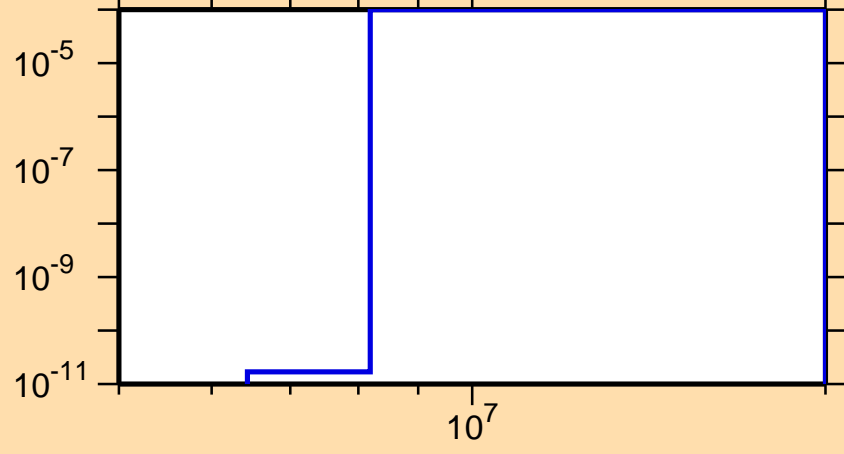
\sigma vs. E for ^{232}\text{Np}(n,np)
