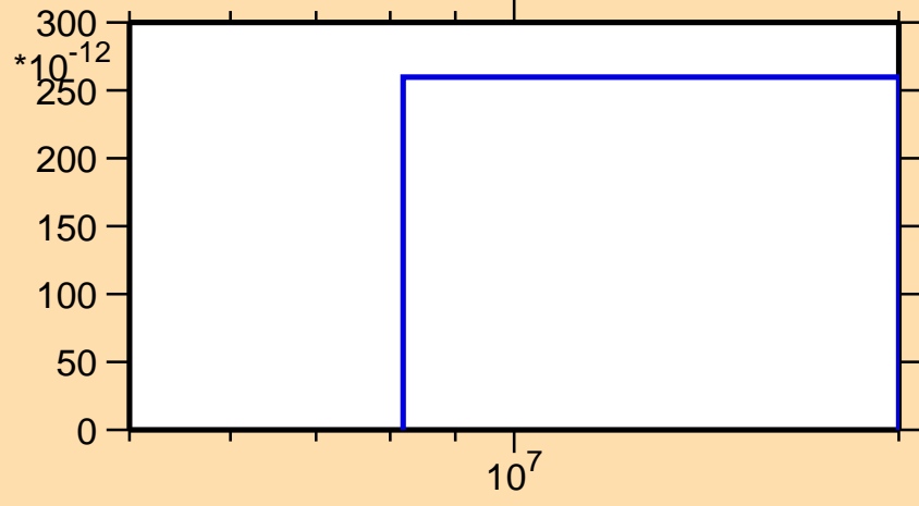
\sigma vs. E for ^{232}\text{Np}(n,2n\alpha)
