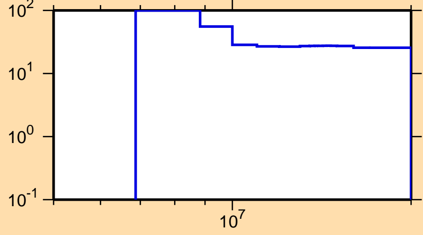
\Delta\sigma/\sigma vs. E for ^{233}\text{Np}(n,2n)
