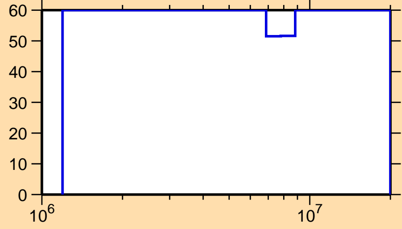
\Delta\sigma/\sigma vs. E for ^{233}\text{Np}(n,ncont.)
