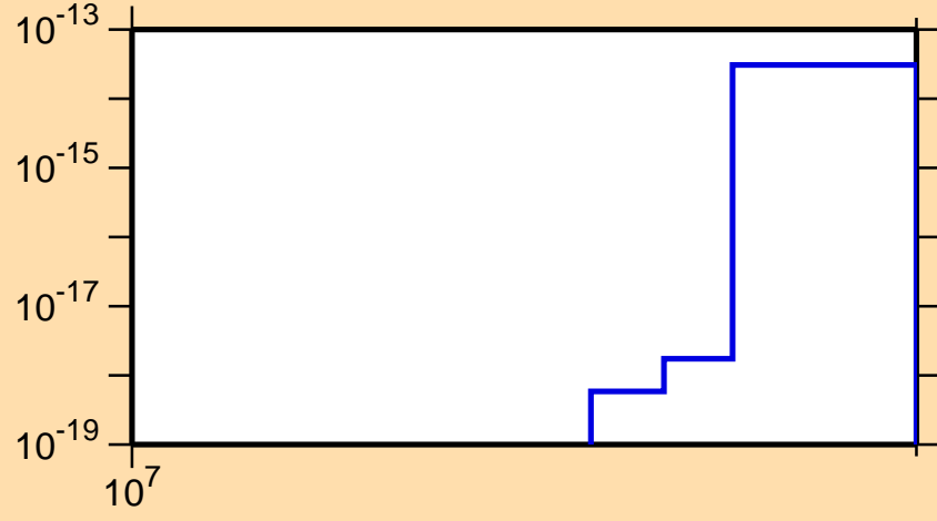
\sigma vs. E for ^{233}\text{Np}(\text{mt } 11)
