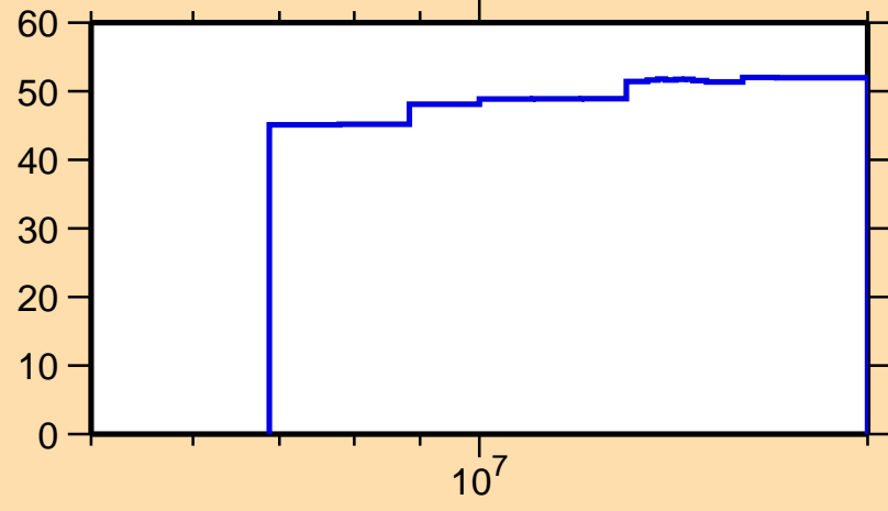
\Delta\sigma/\sigma vs. E for ^{233}\text{Np}(n,\text{inel.})
