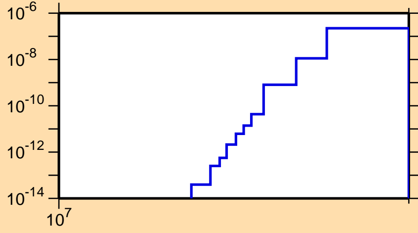
\sigma vs. E for ^{233}\text{Np}(n,\text{nd})
