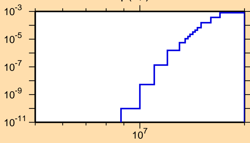
\sigma vs. E for ^{233}\text{Np}(n,t)
