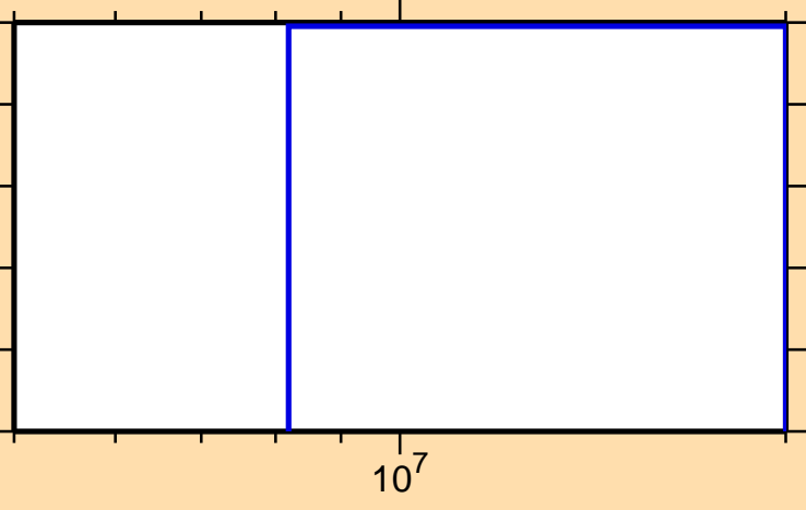
\sigma vs. E for ^{233}\text{Np}(n,3n)
