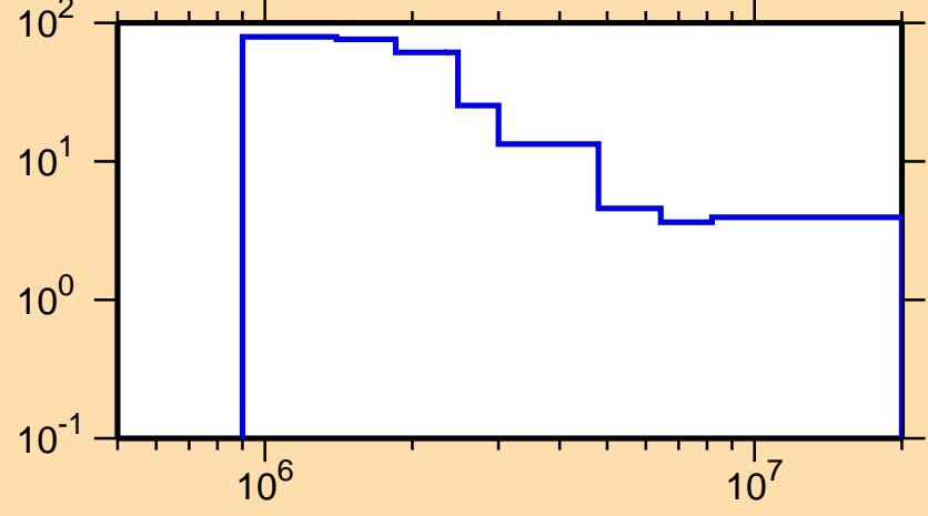
\Delta\sigma/\sigma vs. E for ^{233}\text{Np}(n,f)
