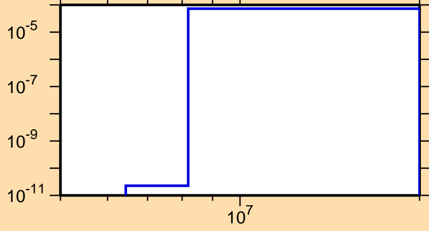
\sigma vs. E for ^{233}\text{Np}(n,np)
