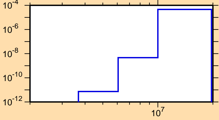
\sigma vs. E for ^{234}\text{Np}(n,n\alpha)
