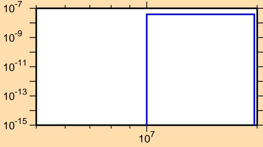
\sigma vs. E for ^{234}\text{Np}(n,\text{nd})
