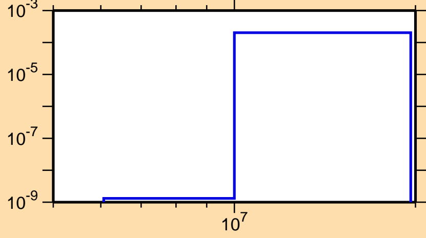
\sigma vs. E for ^{234}\text{Np}(n,np)
