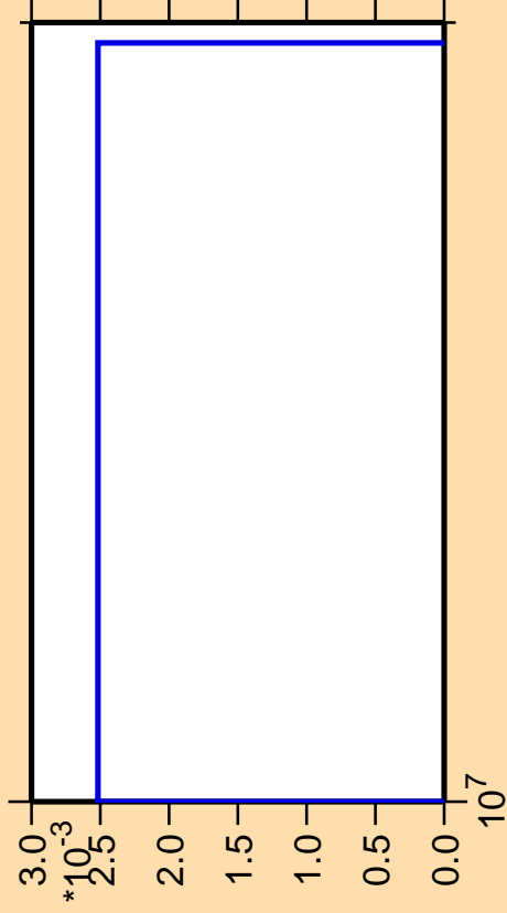
\Delta\sigma/\sigma vs. E for ^{234}\text{Np} (mt 34)
