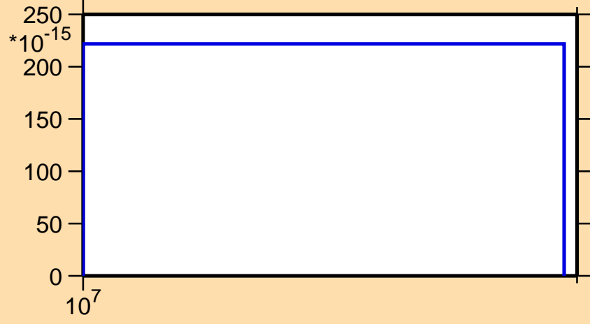
\sigma vs. E for ^{234}\text{Np}(n,p\alpha)
