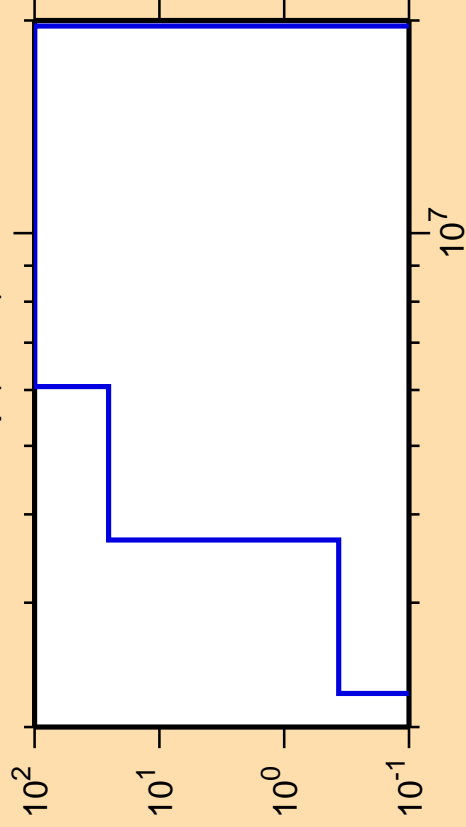
\Delta\sigma/\sigma vs. E for ^{234}\text{Np}(n,n\alpha)
