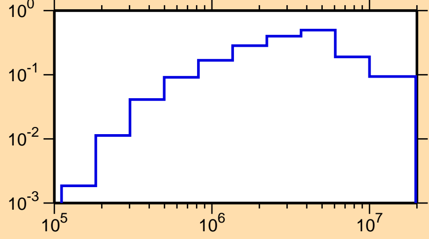
\sigma vs. E for ^{234}\text{Np}(n,n\text{cont.})
