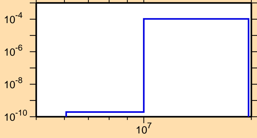
\sigma vs. E for ^{234}\text{Np}(n,t)
