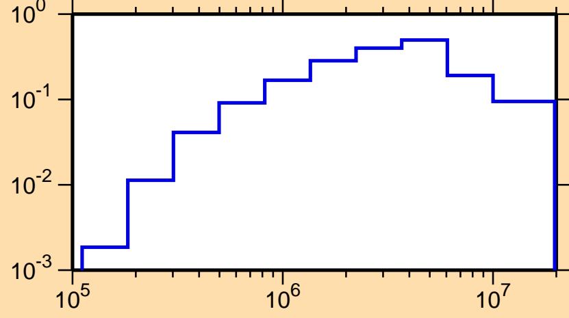
\sigma vs. E for ^{234}\text{Np}(n,\text{inel.})
