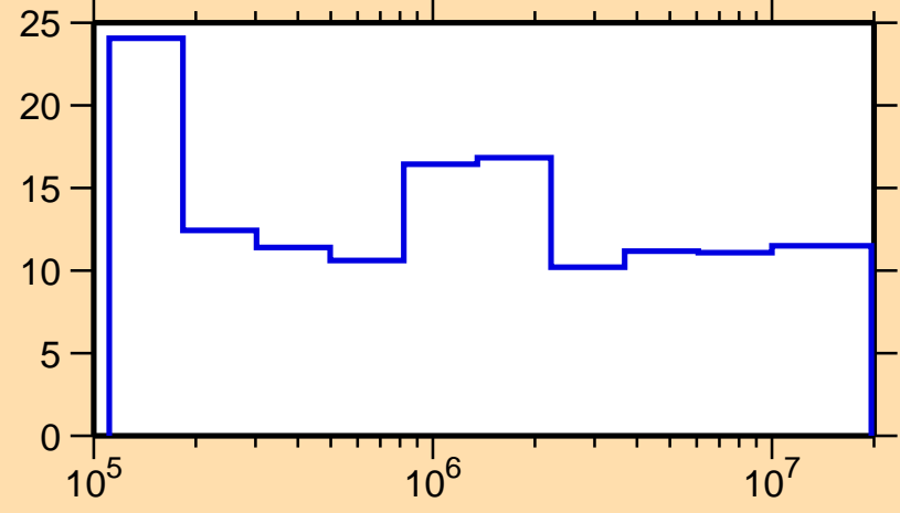
\Delta\sigma/\sigma vs. E for ^{234}\text{Np}(n,n\text{onel.})
