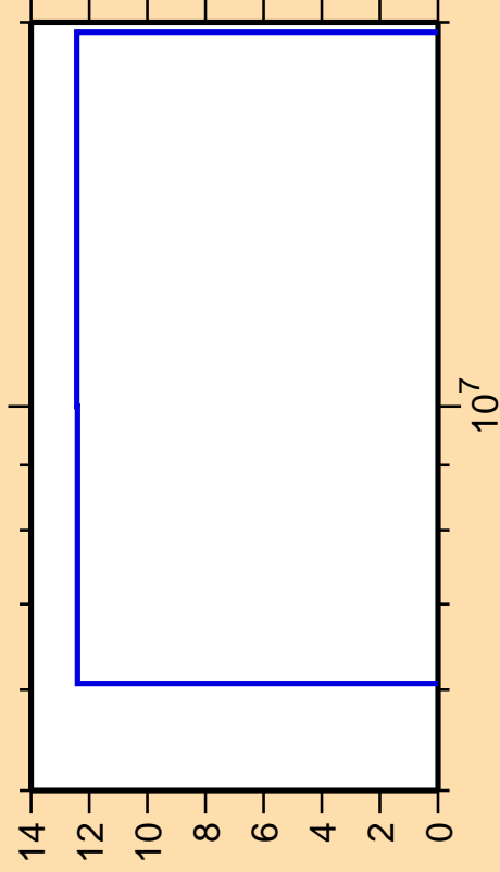
\Delta\sigma/\sigma vs. E for ^{234}\text{Np}(n,f)
