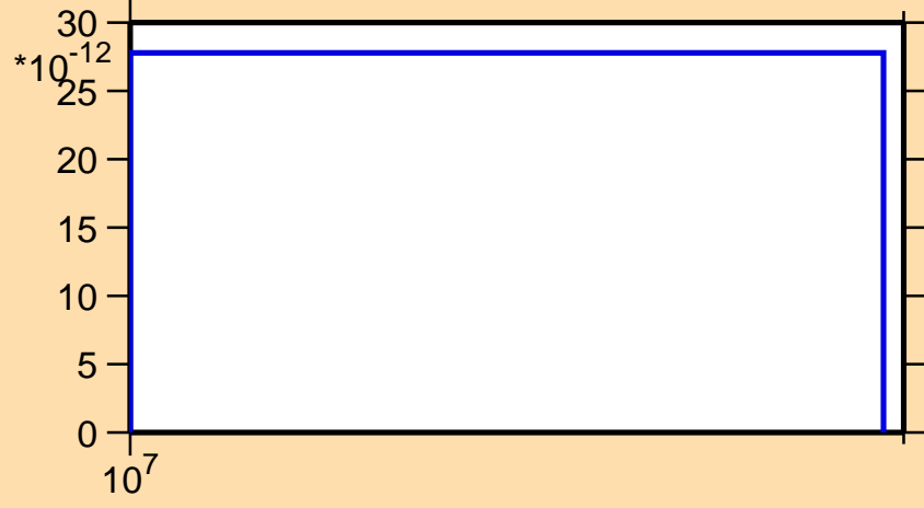
\sigma vs. E for ^{234}\text{Np}(n,\text{He3})
