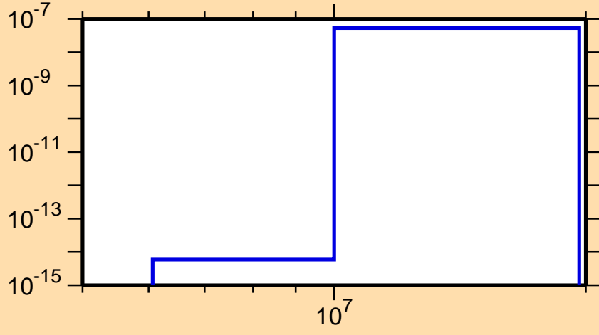
\sigma vs. E for ^{234}\text{Np}(n,2n\alpha)
