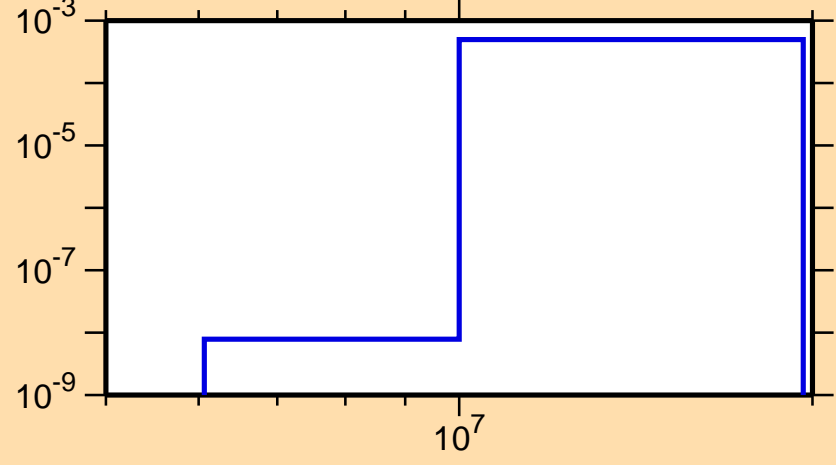
\sigma vs. E for ^{234}\text{Np}(n,d)
