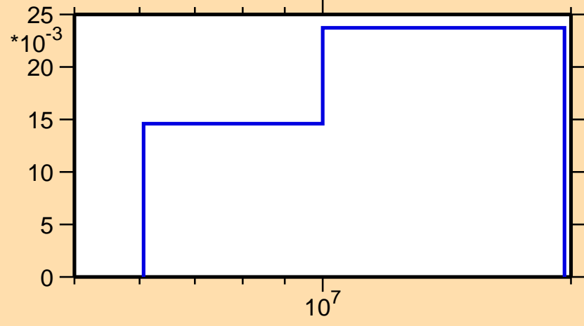
\sigma vs. E for ^{234}\text{Np}(n,2n)
