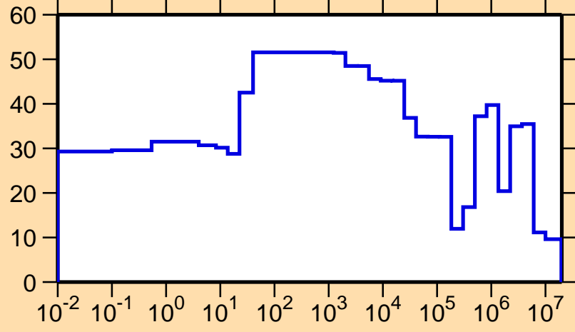
\Delta\sigma/\sigma vs. E for ^{234}\text{Np}(n,el.)
