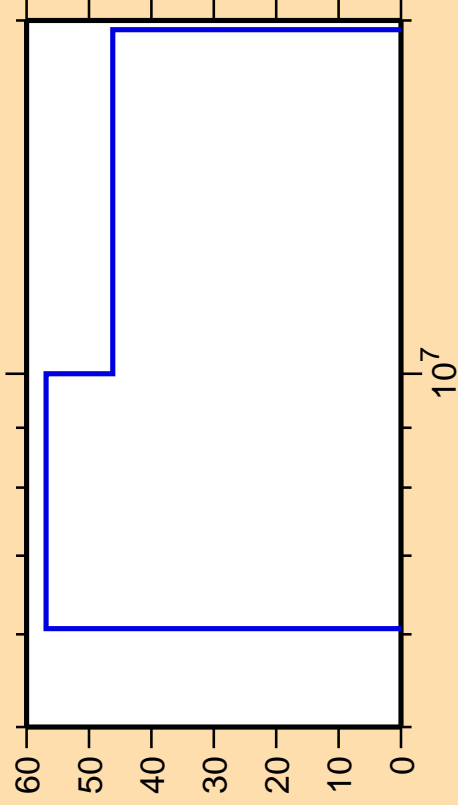
\Delta\sigma/\sigma vs. E for ^{234}\text{Np}(n,t)
