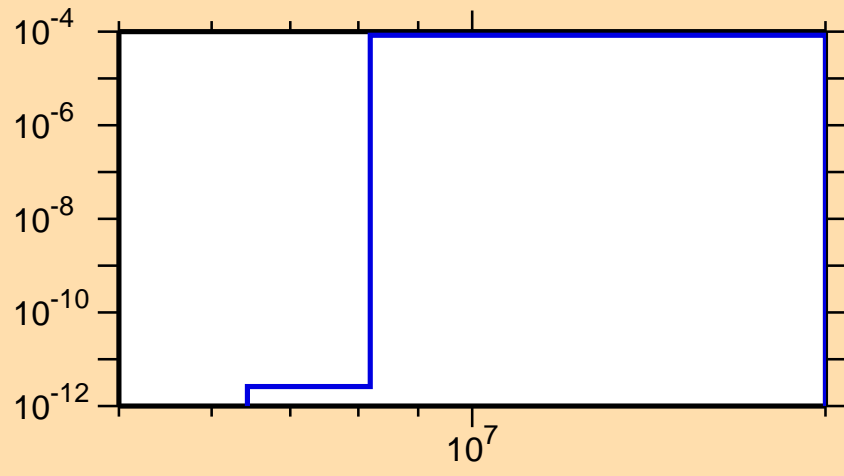
\sigma vs. E for ^{234}\text{Np}(n,t)
