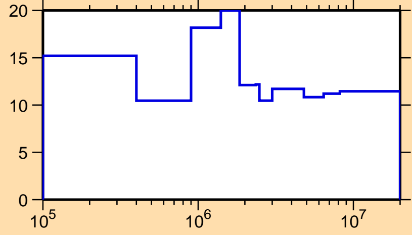
\Delta\sigma/\sigma vs. E for ^{234}\text{Np}(n,n\text{nonel.})
