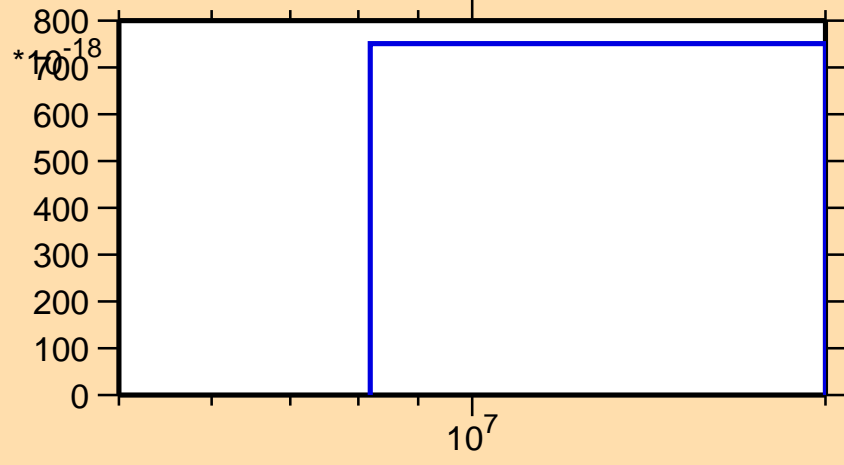
\sigma vs. E for ^{234}\text{Np}(\text{mt } 34)
