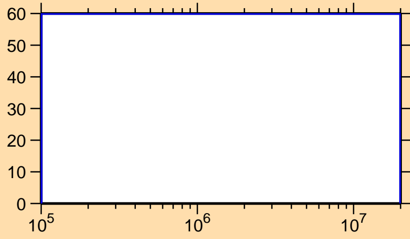
\Delta\sigma/\sigma vs. E for ^{234}\text{Np}(n,inel.)
