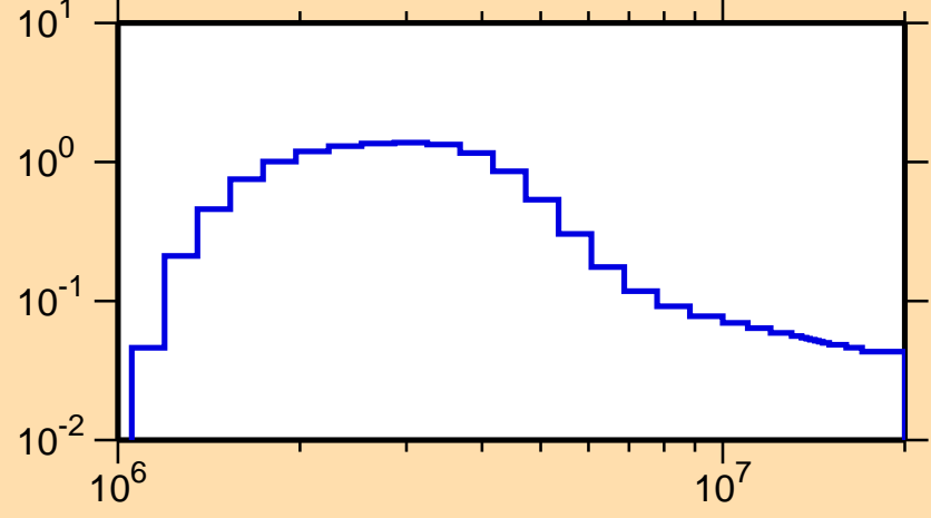
\sigma vs. E for ^{235}\text{Np}(n,n\text{cont.})
