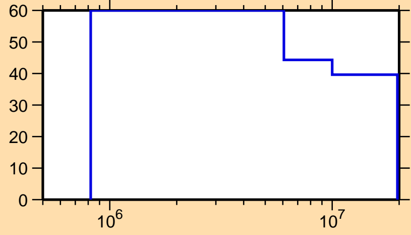
\Delta\sigma/\sigma vs. E for ^{235}\text{Np}(n,inel.)
