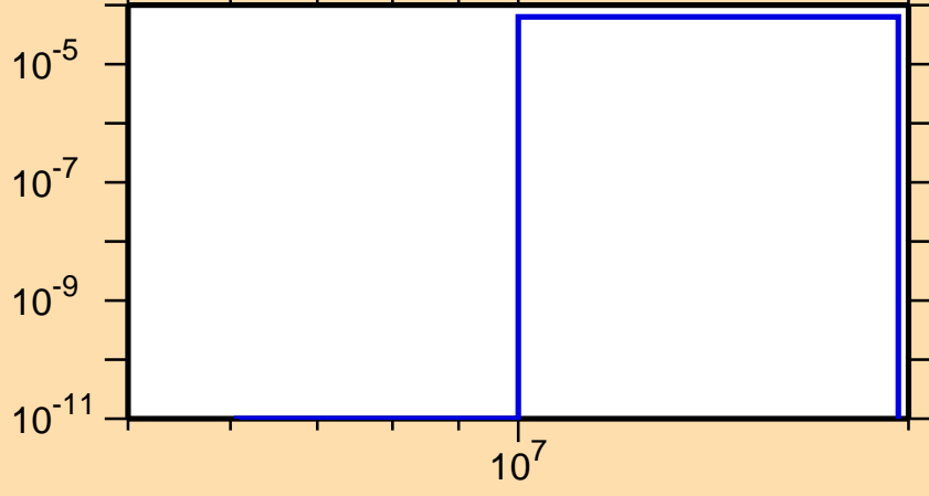
\sigma vs. E for ^{235}\text{Np}(n,t)
