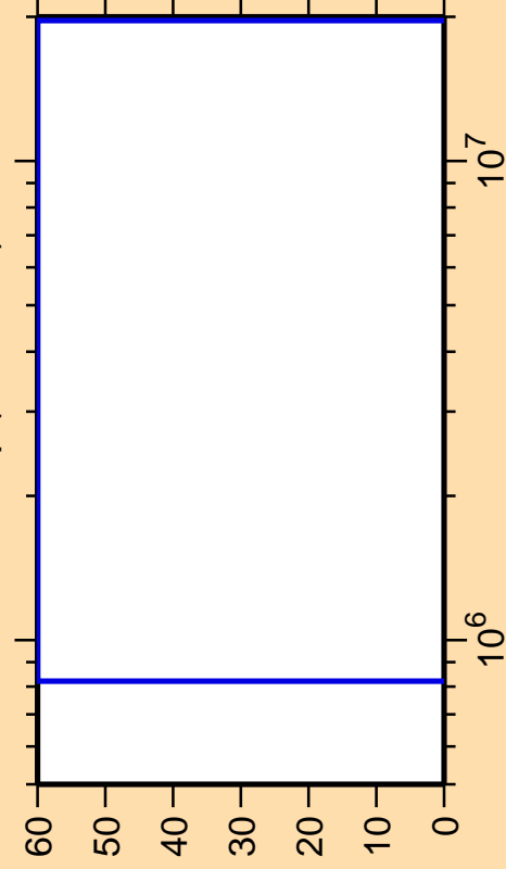
\Delta\sigma/\sigma vs. E for ^{235}\text{Np}(n,ncont.)
