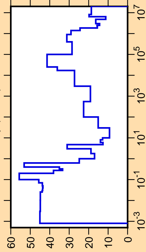
\Delta\sigma/\sigma vs. E for ^{235}\text{Np}(n,\text{tot.})
