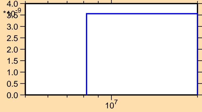
\sigma vs. E for ^{235}\text{Np}(n,2np)
