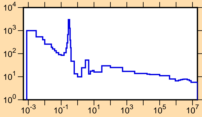
\sigma vs. E for ^{235}\text{Np}(n,\text{tot.})
