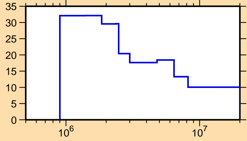
\Delta\sigma/\sigma vs. E for ^{235}\text{Np}(n,n\text{onel.})
