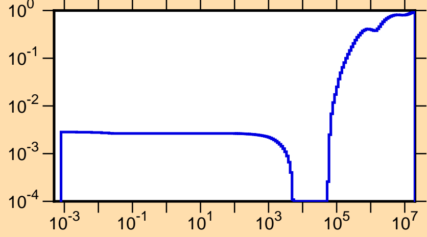
\mu vs. E for ^{236}\text{Np}(\text{mt251})
