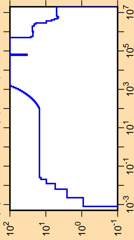
\Delta\mu/\mu vs. E for ^{236}\text{Np}(\text{mt251})
