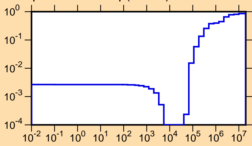
\mu vs. E for ^{236}\text{Np}(\text{mt251})
