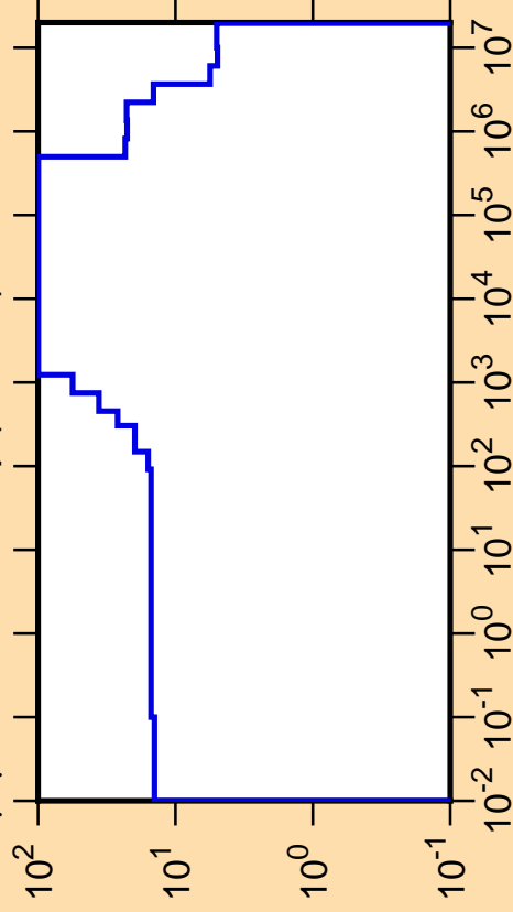
\Delta\mu/\mu vs. E for ^{236}\text{Np}(\text{mt251})
