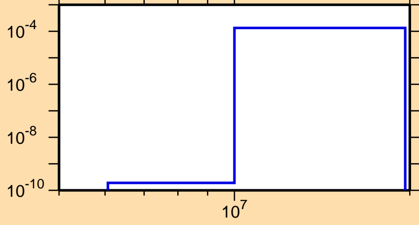
\sigma vs. E for ^{236}\text{Np}(n,np)
