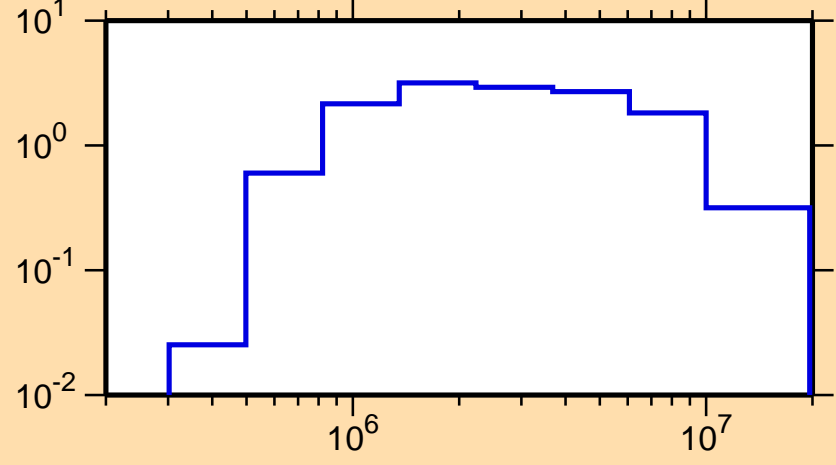
\sigma vs. E for ^{236}\text{Np}(n,n\text{cont.})
