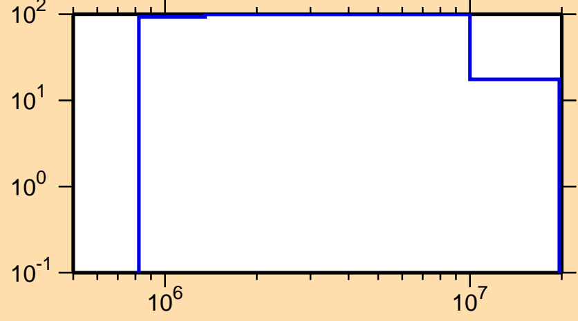
\Delta\sigma/\sigma vs. E for ^{236}\text{Np}(n,f)
