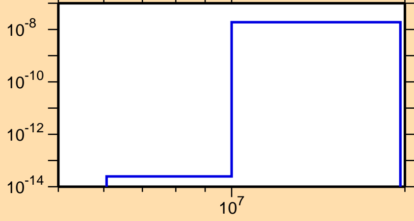
\sigma vs. E for ^{236}\text{Np}(n,2n\alpha)
