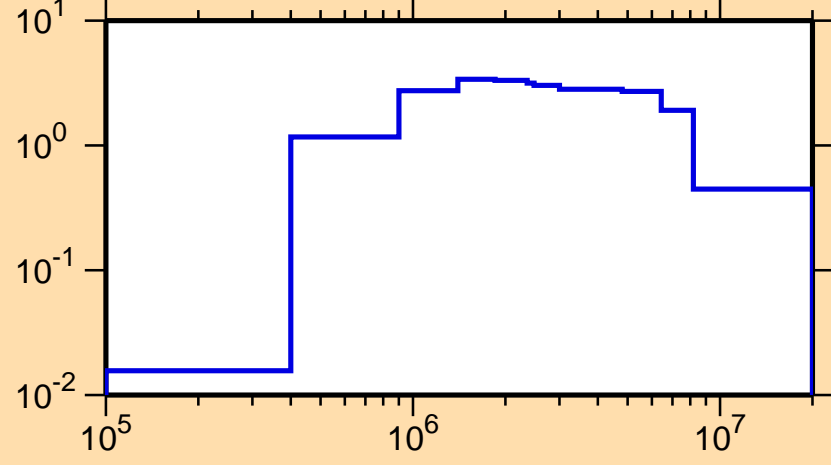
\sigma vs. E for ^{236}\text{Np}(n,\text{inel.})
