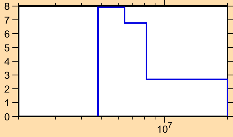
\Delta\sigma/\sigma vs. E for ^{236}\text{Np}(n,\text{tot.})
