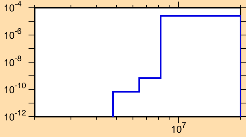
\sigma vs. E for ^{236}\text{Np}(n,\alpha)
