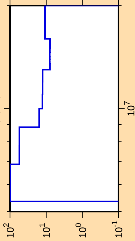
\Delta\sigma/\sigma vs. E for ^{236}\text{Np}(n,f)
