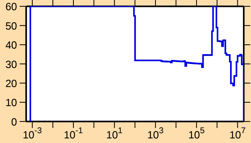
\Delta\sigma/\sigma vs. E for ^{236}\text{Np}(n,\text{el.})
