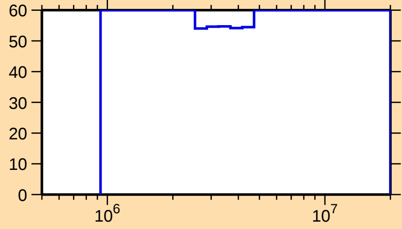
\Delta\sigma/\sigma vs. E for ^{236}\text{Np}(n,\gamma)
