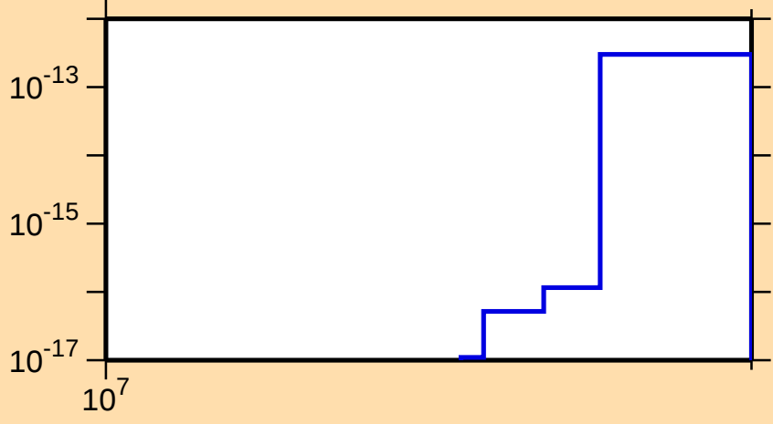
\sigma vs. E for ^{236}\text{Np}(\text{mt 11})
