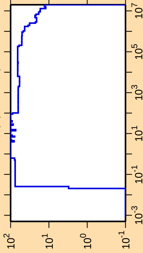
\Delta\sigma/\sigma vs. E for ^{236}\text{Np}(n,\text{nonel.})
