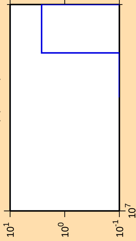
\Delta\sigma/\sigma vs. E for ^{236}\text{Np}(\text{mt 11})
