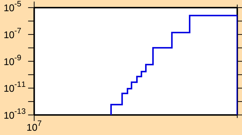
\sigma vs. E for ^{236}\text{Np}(n,nt)
