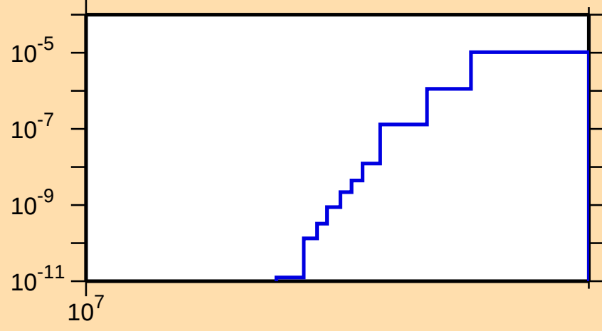
\sigma vs. E for ^{236}\text{Np}(n,2np)
