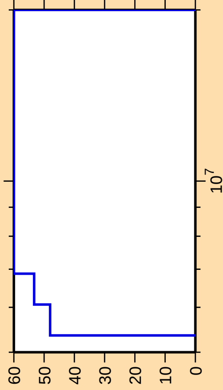
\Delta\sigma/\sigma vs. E for ^{236}\text{Np}(n,n\text{cont.})
