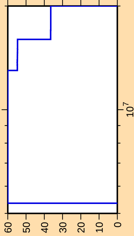
\Delta\sigma/\sigma vs. E for ^{236}\text{Np}(n,\alpha)
