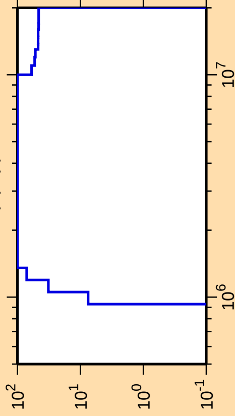
\Delta\sigma/\sigma vs. E for ^{236}\text{Np}(n,p)
