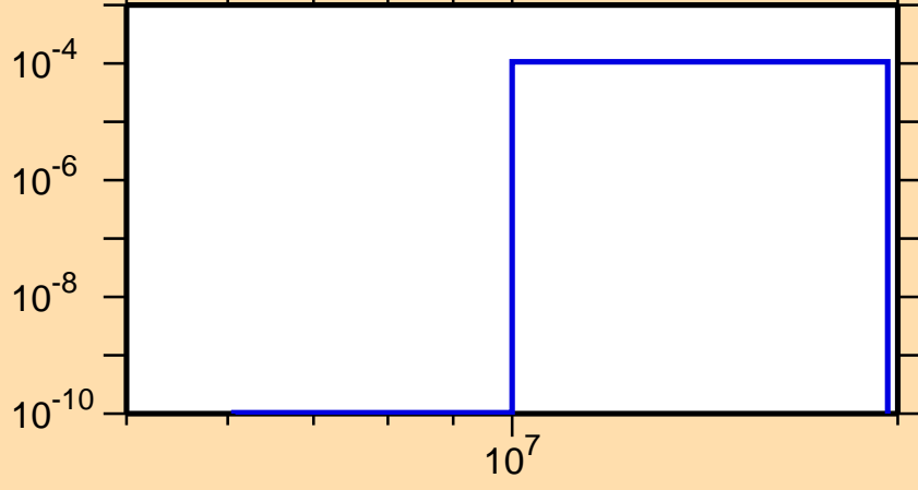
\sigma vs. E for ^{236}\text{Np}(n,t)
