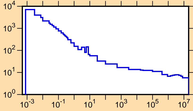
\sigma vs. E for ^{236}\text{Np}(n,\text{tot.})
