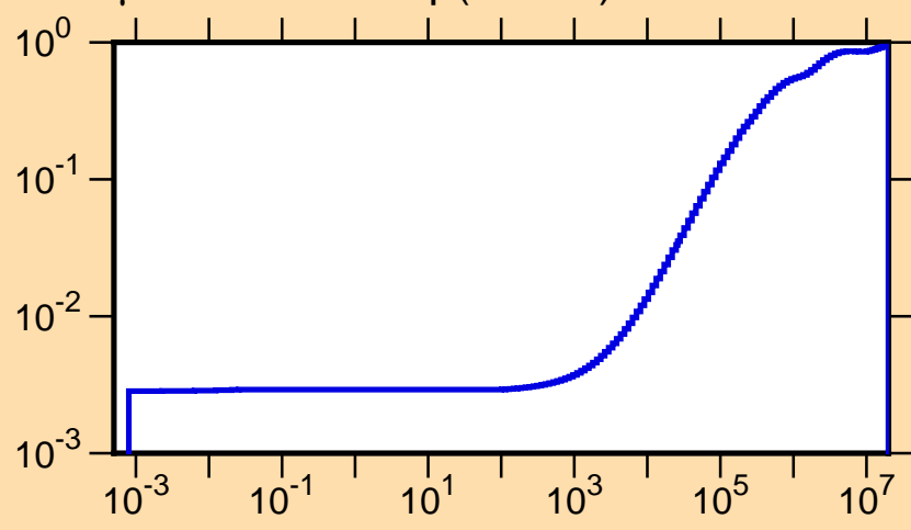
\mu vs. E for ^{237}\text{Np}(\text{mt251})
