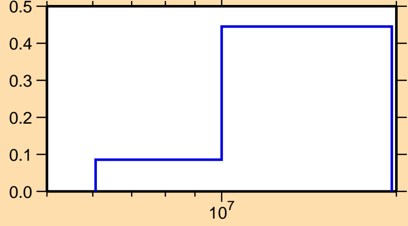
\sigma vs. E for ^{237}\text{Np}(n,2n)
