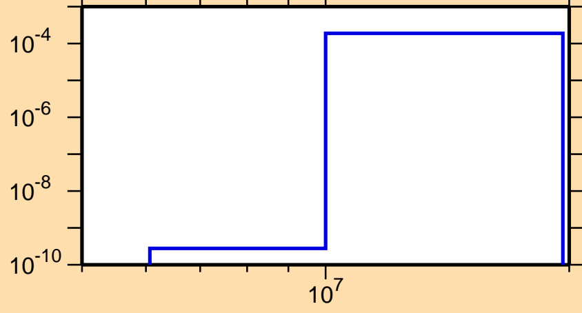
\sigma vs. E for ^{237}\text{Np}(n,np)
