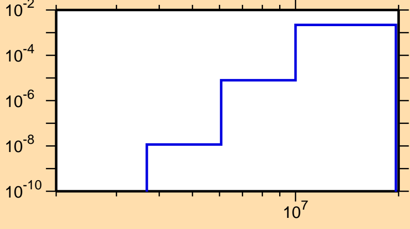
\sigma vs. E for ^{237}\text{Np}(n,p)
