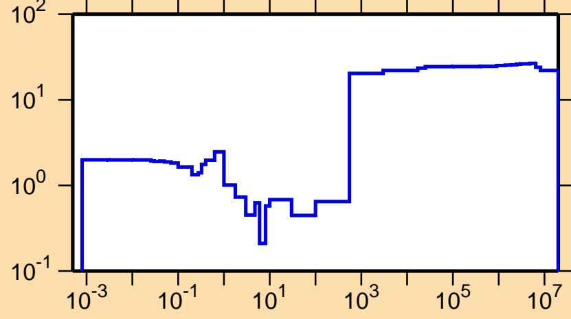
\Delta\sigma/\sigma vs. E for ^{237}\text{Np}(n,\gamma)
