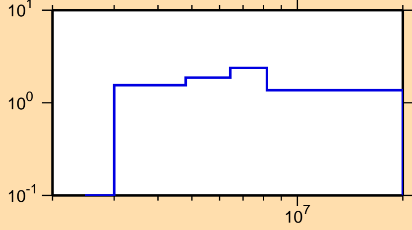
\Delta\sigma/\sigma vs. E for ^{237}\text{Np}(n,p)
