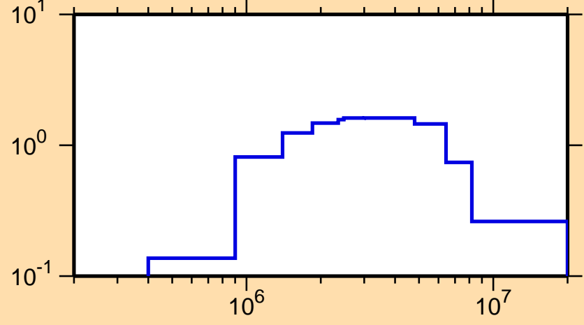
\sigma vs. E for ^{237}\text{Np}(n,n\text{cont.})
