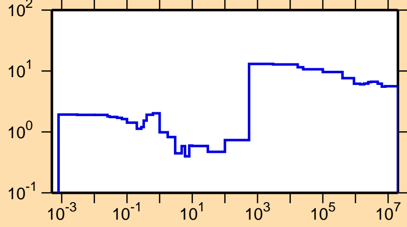
\Delta\sigma/\sigma vs. E for ^{237}\text{Np}(n,\text{tot.})
