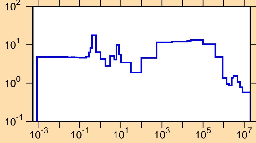
\Delta\sigma/\sigma vs. E for ^{237}\text{Np}(n,f)
