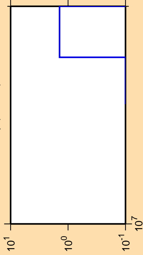
\Delta\sigma/\sigma vs. E for ^{238}\text{Np}(\text{mt } 11)
