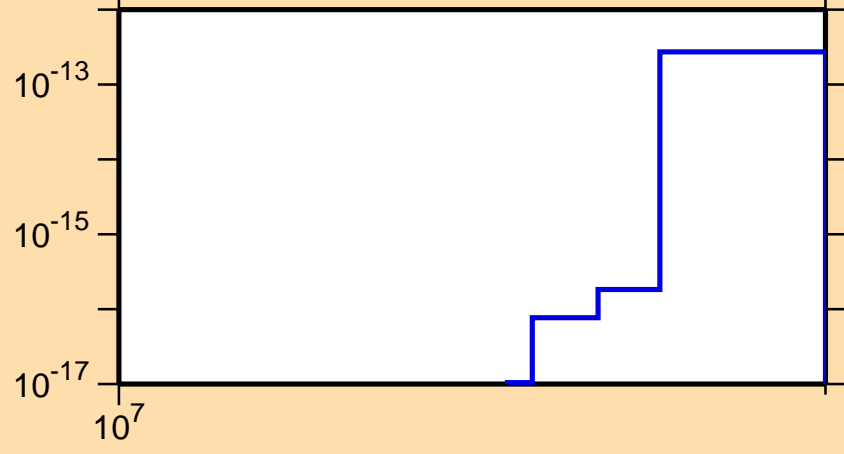
\sigma vs. E for ^{238}\text{Np}(\text{mt } 11)
