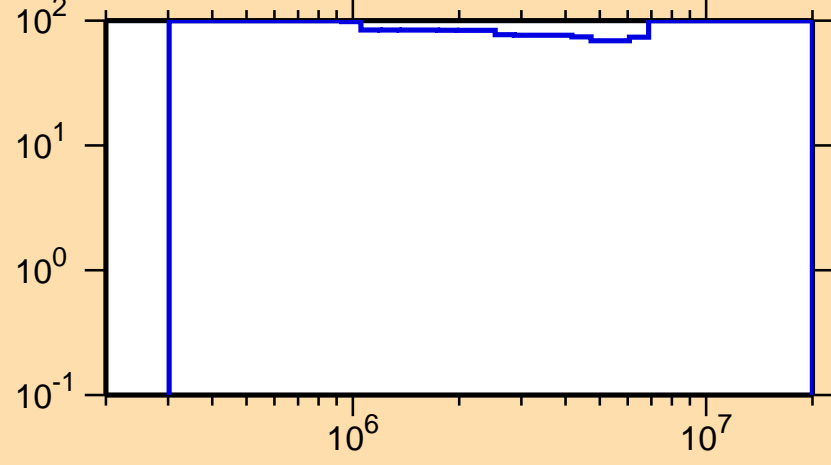
\Delta\sigma/\sigma vs. E for ^{238}\text{Np}(n,n\text{cont.})
