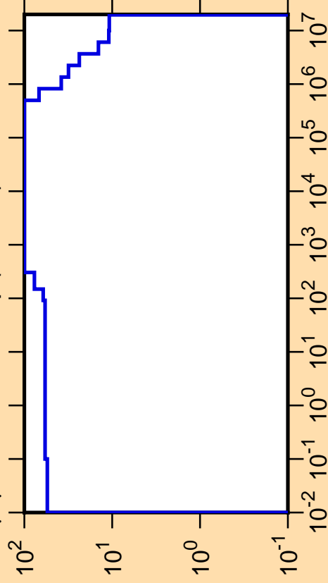
\Delta\mu/\mu vs. E for ^{238}\text{Np}(\text{mt251})
