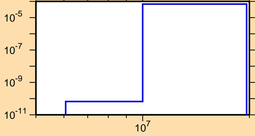
\sigma vs. E for ^{238}\text{Np}(n,t)
