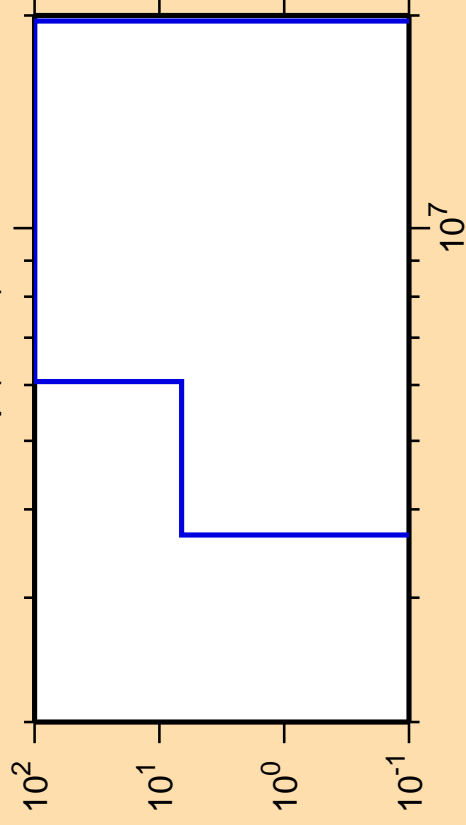
\Delta\sigma/\sigma vs. E for ^{238}\text{Np}(n,n\alpha)
