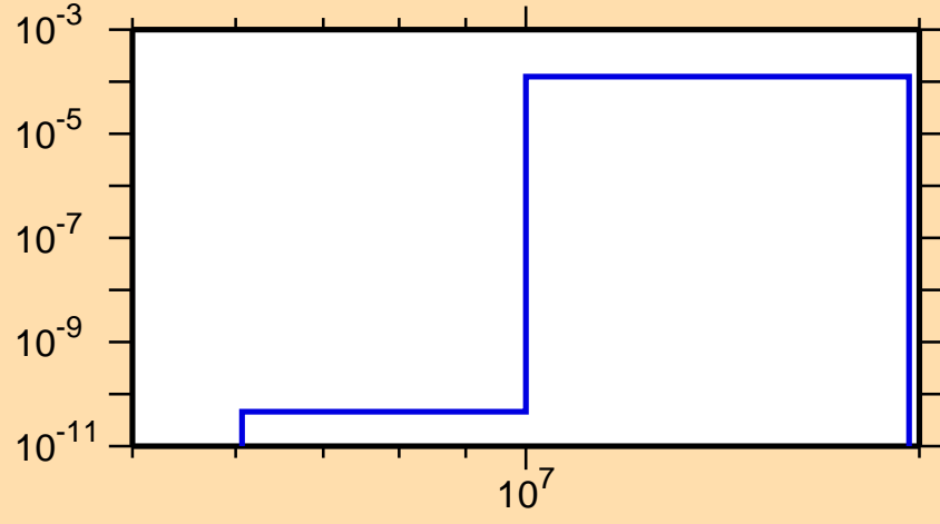
\sigma vs. E for ^{238}\text{Np}(n,np)
