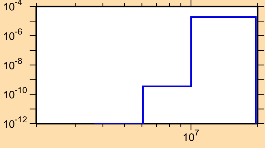
\sigma vs. E for ^{238}\text{Np}(n,n\alpha)
