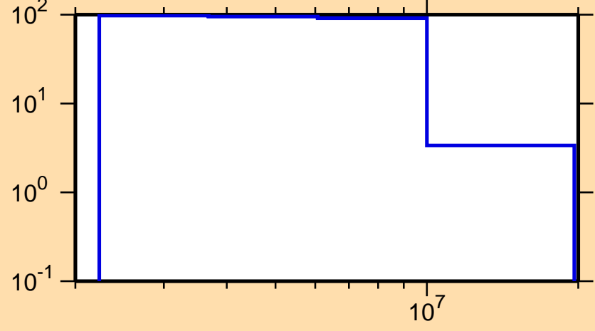
\Delta\sigma/\sigma vs. E for ^{238}\text{Np}(n,n_1)
