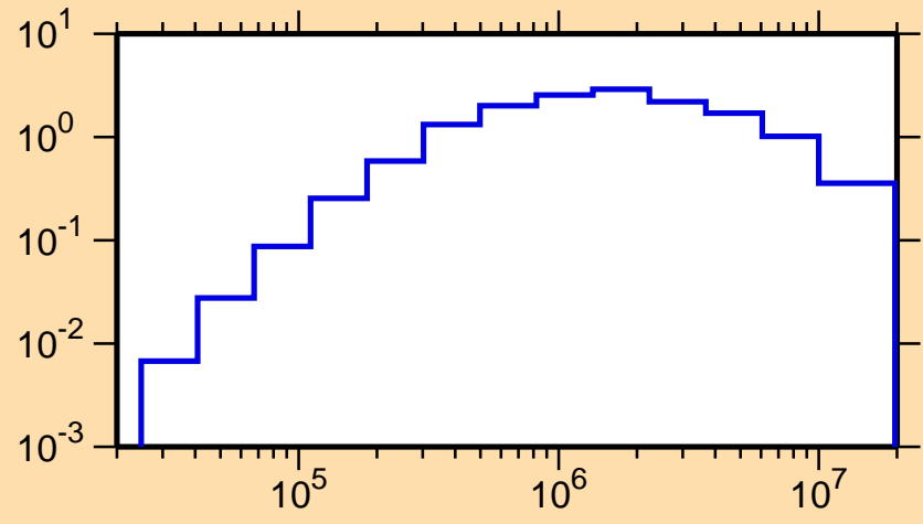
\sigma vs. E for ^{238}\text{Np}(n,\text{inel.})
