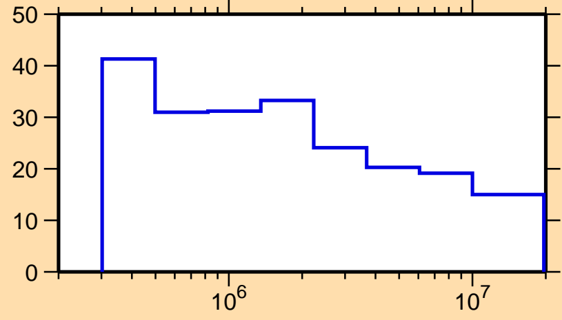
\Delta\sigma/\sigma vs. E for ^{238}\text{Np}(n,n\text{nonel.})
