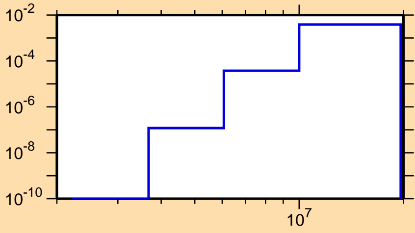
\sigma vs. E for ^{238}\text{Np}(n,p)
