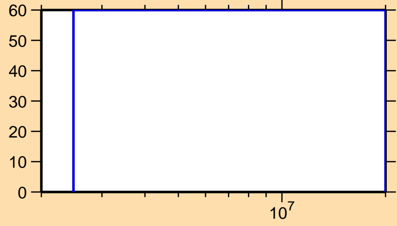
\Delta\sigma/\sigma vs. E for ^{238}\text{Np}(n,ncont.)
