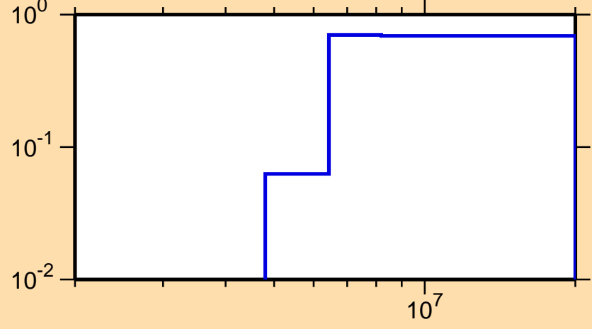
\sigma vs. E for ^{238}\text{Np}(n,2n)
