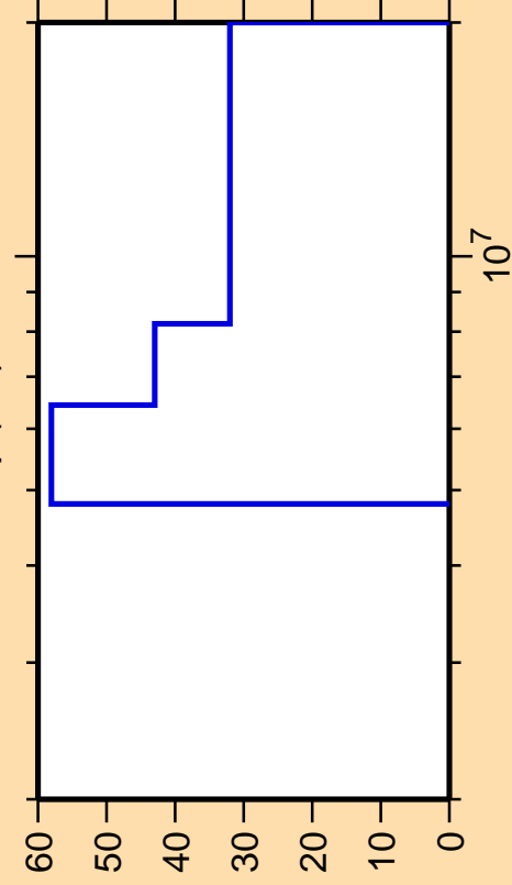
\Delta\sigma/\sigma vs. E for ^{238}\text{Np}(n,f)
