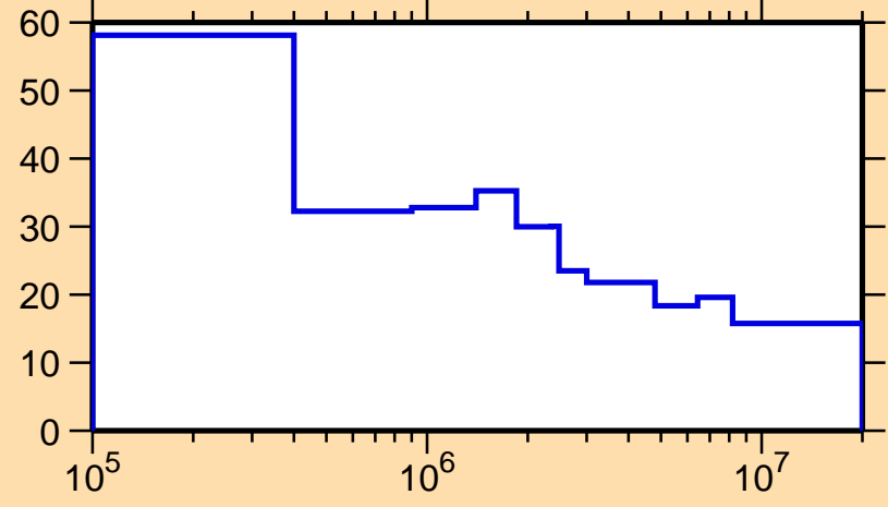
\Delta\sigma/\sigma vs. E for ^{238}\text{Np}(n,n\text{onel.})
