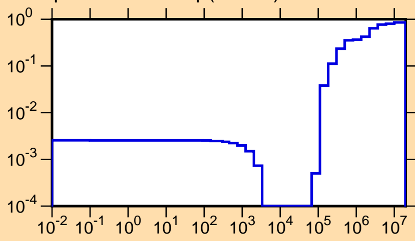
\mu vs. E for ^{239}\text{Np}(\text{mt251})
