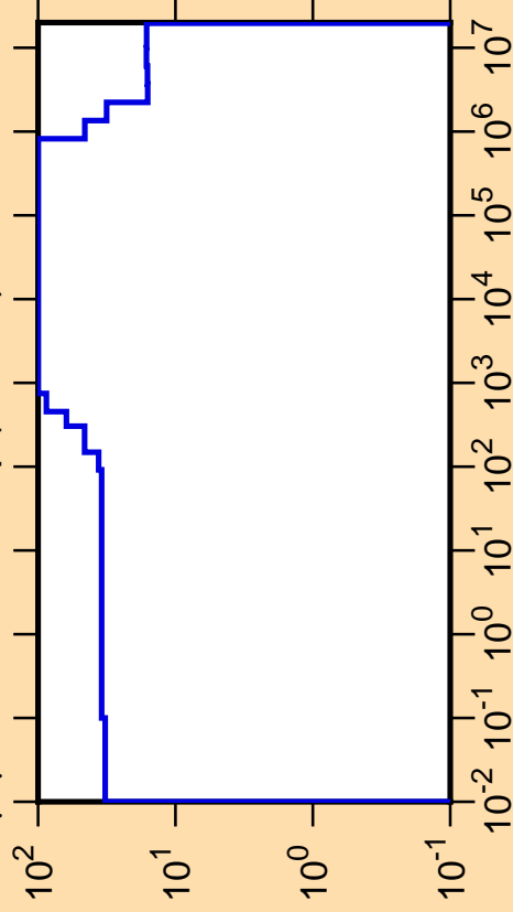
\Delta\mu/\mu vs. E for ^{239}\text{Np}(\text{mt251})
