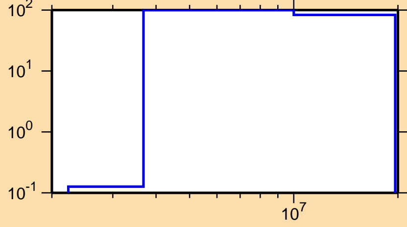
\Delta\sigma/\sigma vs. E for ^{239}\text{Np}(n,p)
