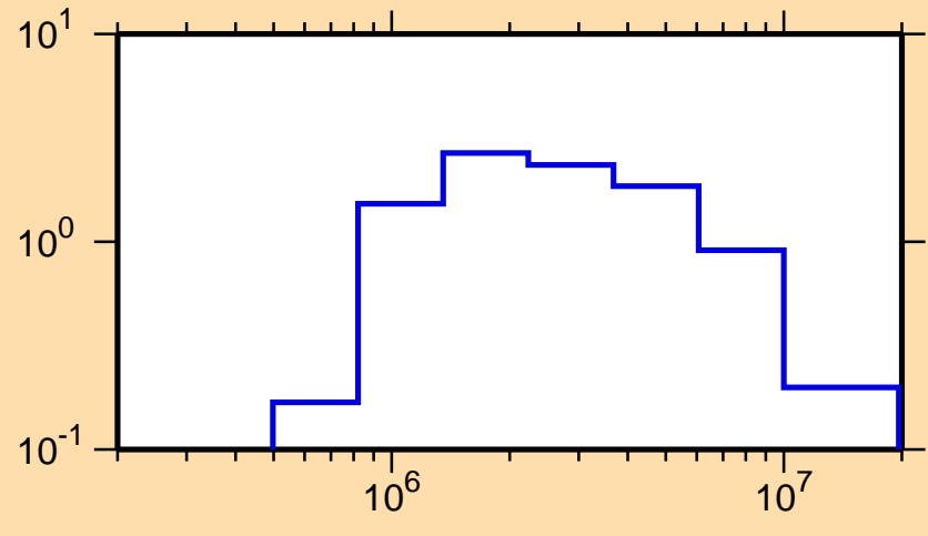
\sigma vs. E for ^{239}\text{Np}(n,n\text{cont.})
