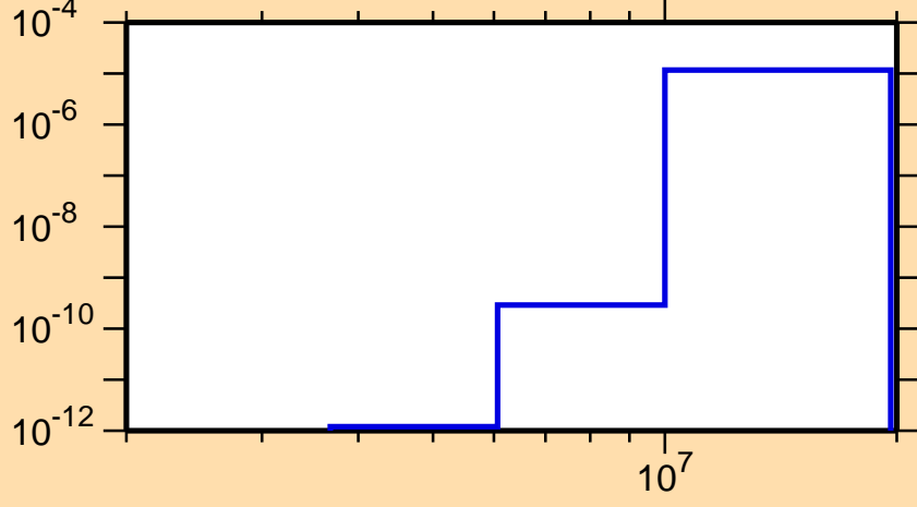
\sigma vs. E for ^{239}\text{Np}(n,n\alpha)
