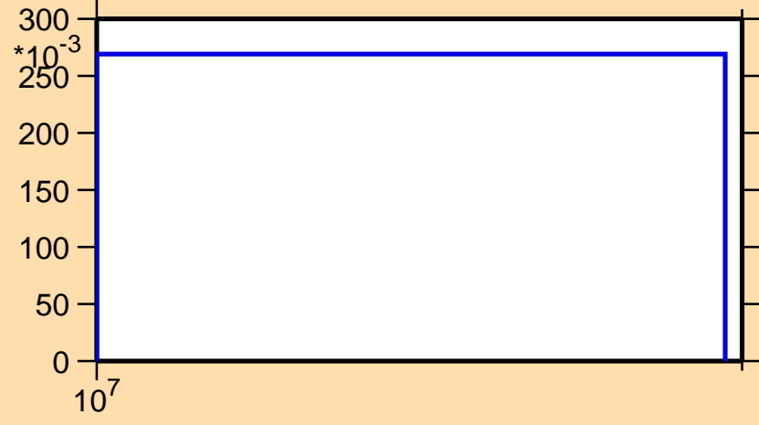
\sigma vs. E for ^{239}\text{Np}(n,3n)
