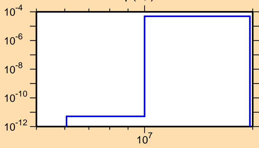
\sigma vs. E for ^{239}\text{Np}(n,t)
