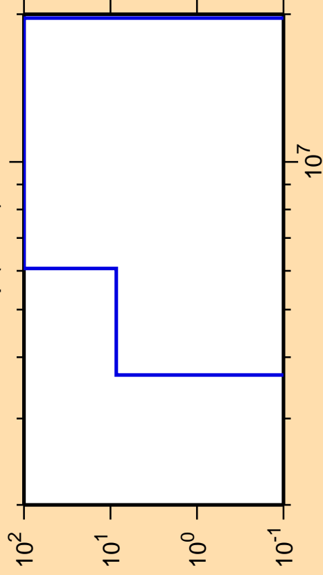
\Delta\sigma/\sigma vs. E for ^{239}\text{Np}(n,n\alpha)
