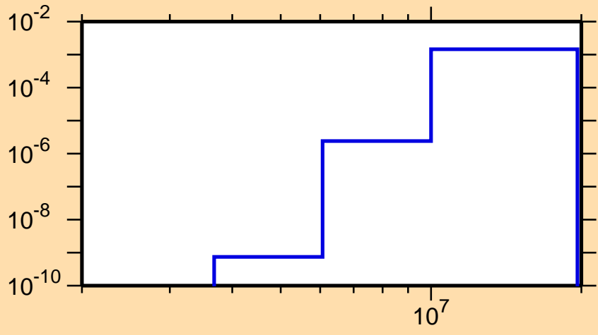
\sigma vs. E for ^{239}\text{Np}(n,p)
