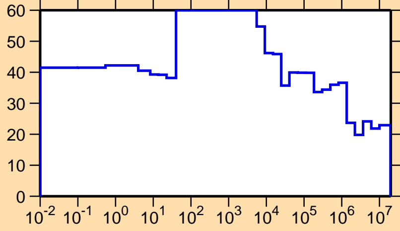
\Delta\sigma/\sigma vs. E for ^{239}\text{Np}(n,el.)
