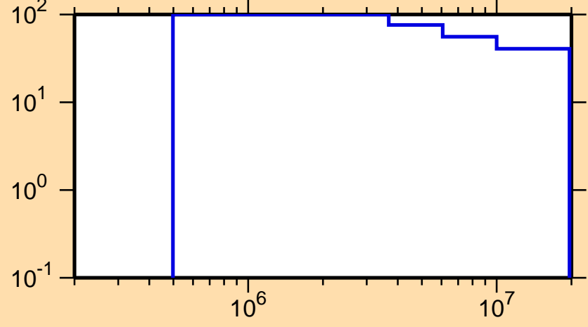
\Delta\sigma/\sigma vs. E for ^{239}\text{Np}(n,f)
