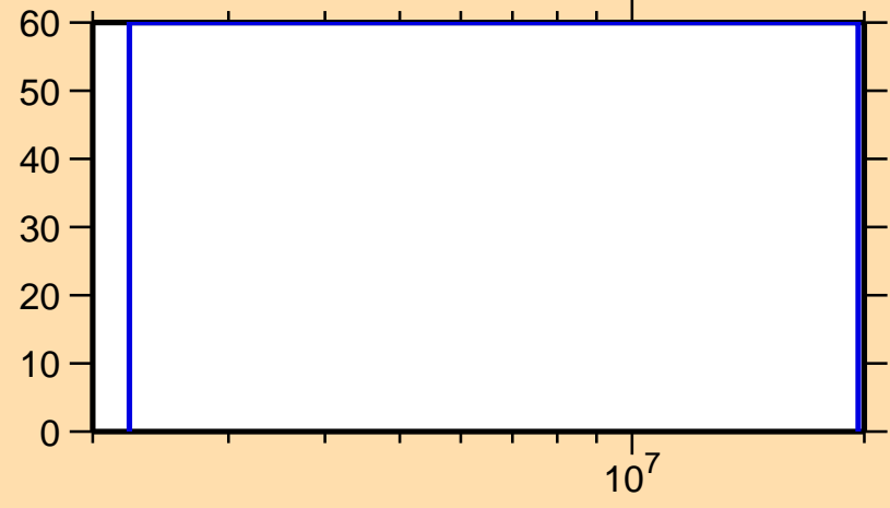
\Delta\sigma/\sigma vs. E for ^{239}\text{Np}(n,ncont.)
