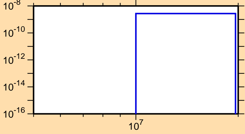
\sigma vs. E for ^{239}\text{Np}(n,2n\alpha)
