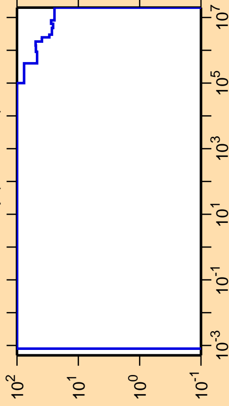
\Delta\sigma/\sigma vs. E for ^{239}\text{Np}(n,\text{nonel.})
