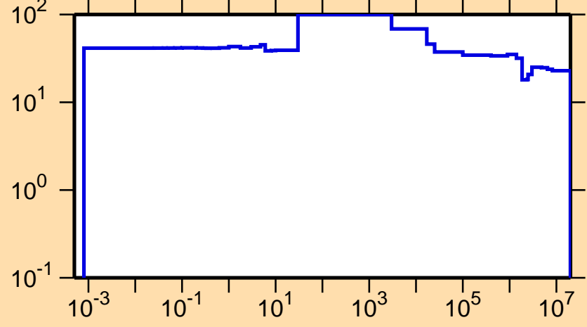
\Delta\sigma/\sigma vs. E for ^{239}\text{Np}(n,\text{el.})
