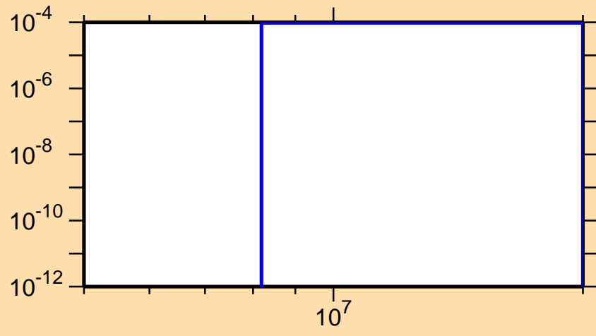
\sigma vs. E for ^{239}\text{Np}(n,d)
