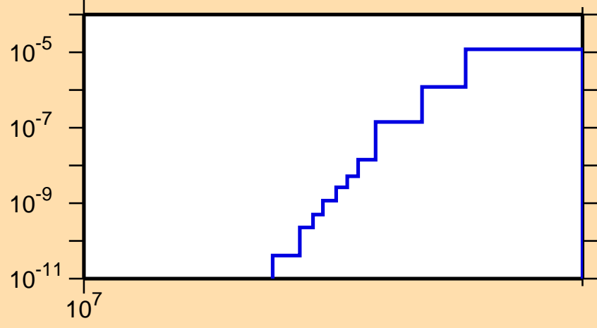
\sigma vs. E for ^{240}\text{Np}(n,nd)
