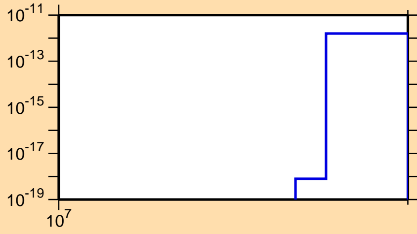
\sigma vs. E for ^{240}\text{Np}(\text{mt } 11)
