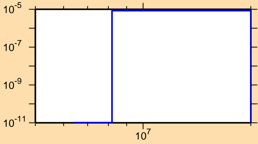
\sigma vs. E for ^{240}\text{Np}(n,\alpha)
