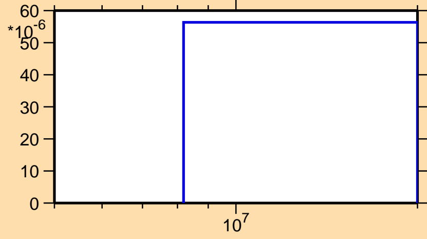
\sigma vs. E for ^{240}\text{Np}(n,np)
