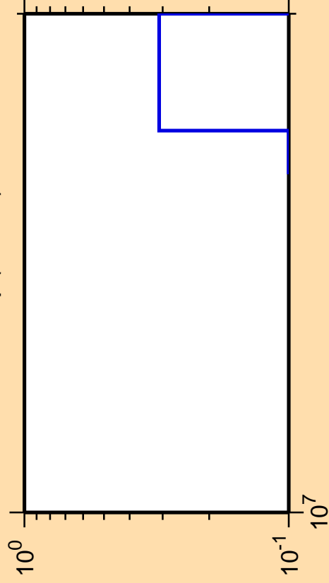
\Delta\sigma/\sigma vs. E for ^{240}\text{Np} (mt 42)
