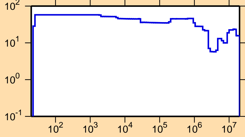
\Delta\sigma/\sigma vs. E for ^{240}\text{Np}(n,\text{el.})
