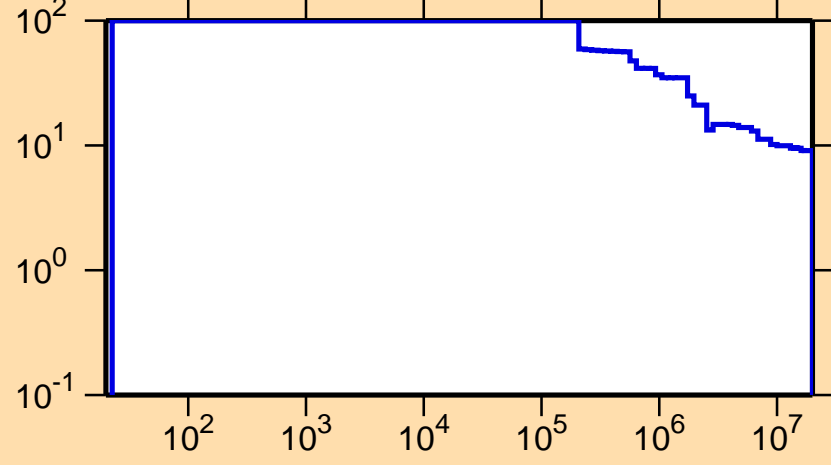
\Delta\sigma/\sigma vs. E for ^{240}\text{Np}(n,\text{nonel.})
