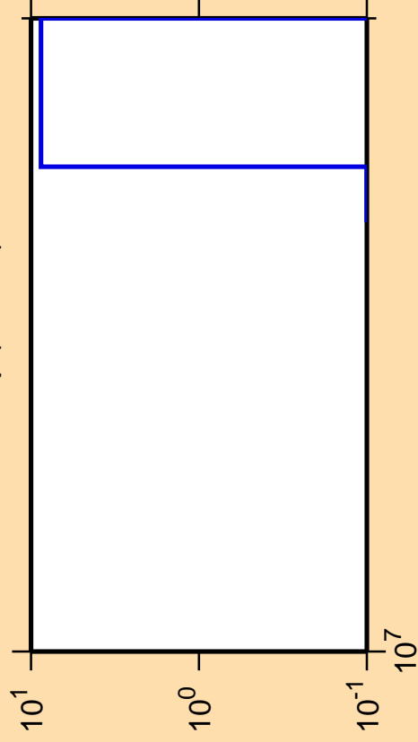
\Delta\sigma/\sigma vs. E for ^{240}\text{Np}(\text{mt } 11)
