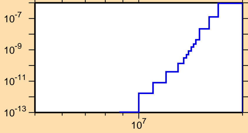
\sigma vs. E for ^{240}\text{Np}(n,2n\alpha)
