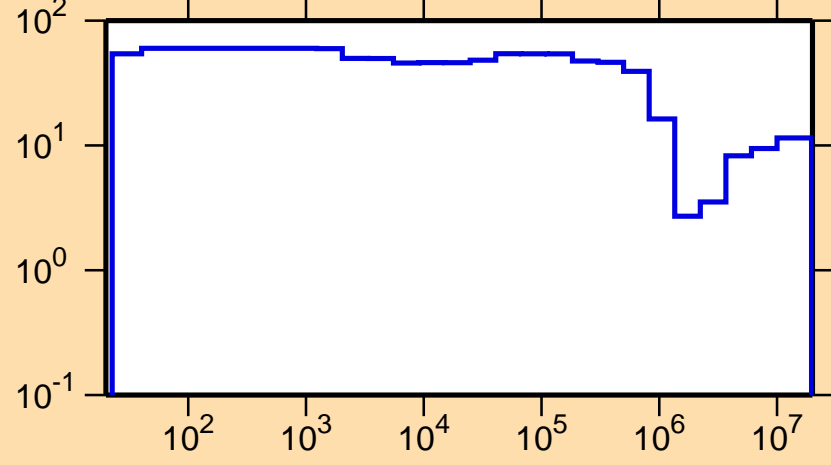
\Delta\sigma/\sigma vs. E for ^{240}\text{Np}(n,\text{tot.})
