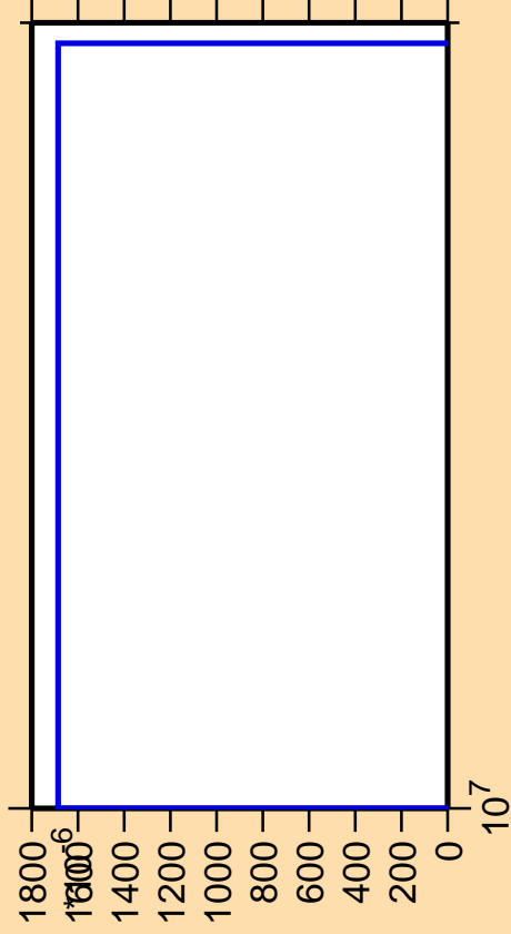
\Delta\sigma/\sigma vs. E for ^{240}\text{Np} (mt 42)
