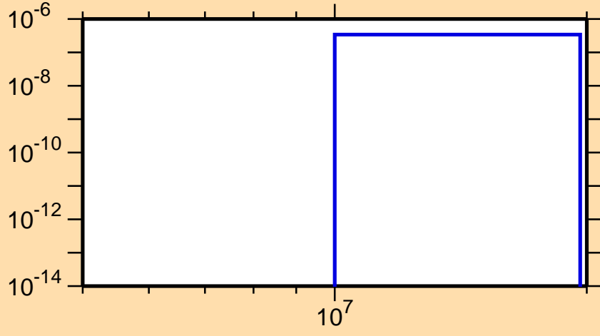
\sigma vs. E for ^{240}\text{Np}(n,\text{nd})
