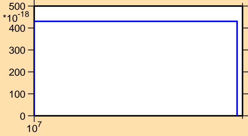
\sigma vs. E for ^{240}\text{Np} (mt 42)
