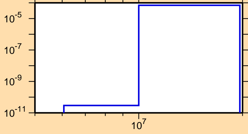
\sigma vs. E for ^{240}\text{Np}(n,t)
