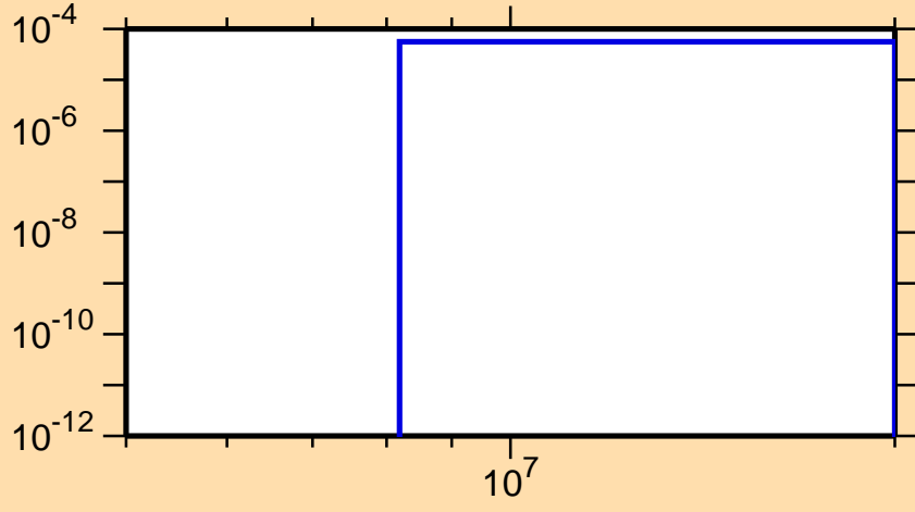
\sigma vs. E for ^{240}\text{Np}(n,t)
