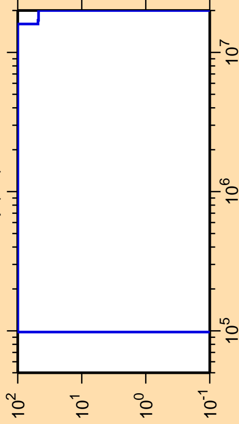
\Delta\sigma/\sigma vs. E for ^{241}\text{Np}(n,f)
