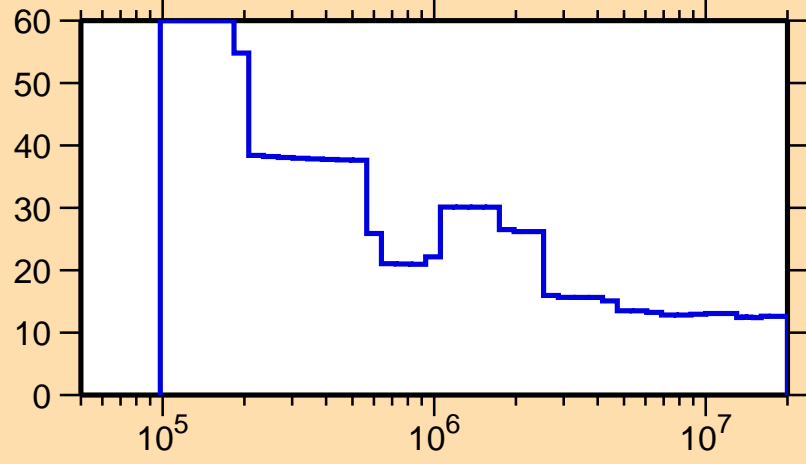
\Delta\sigma/\sigma vs. E for ^{241}\text{Np}(n,n\text{nonel.})
