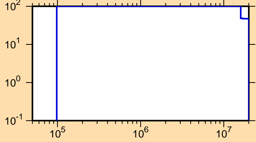
\Delta\sigma/\sigma vs. E for ^{241}\text{Np}(n,f)
