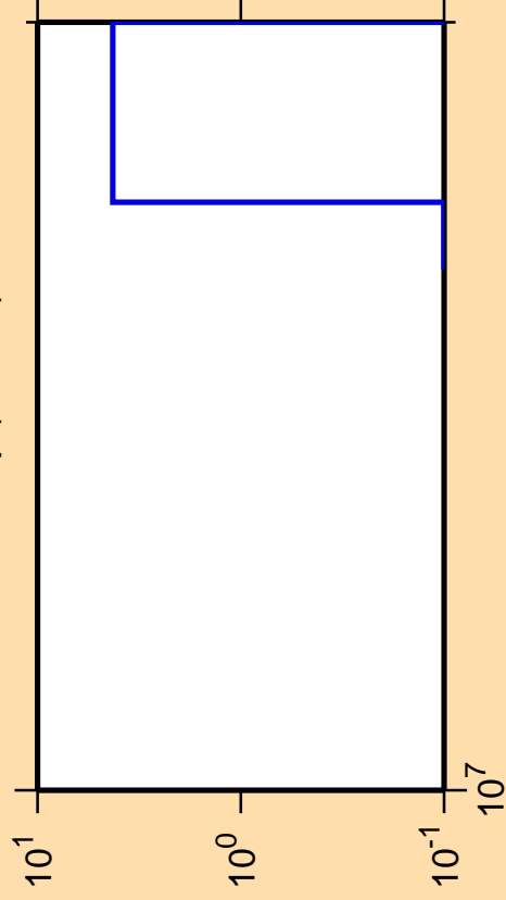
\Delta\sigma/\sigma vs. E for ^{241}\text{Np}(\text{mt } 11)
