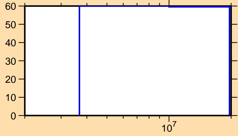
\Delta\sigma/\sigma vs. E for ^{241}\text{Np}(n,ncont.)
