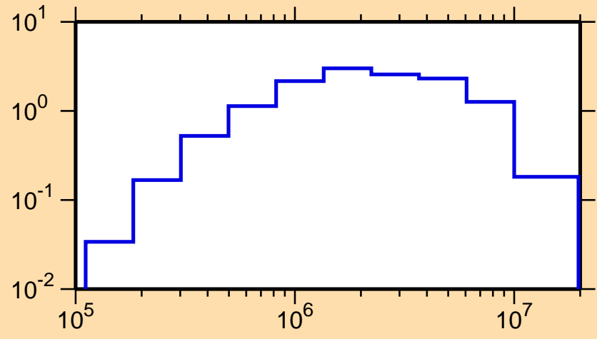
\sigma vs. E for ^{241}\text{Np}(n,n\text{cont.})
