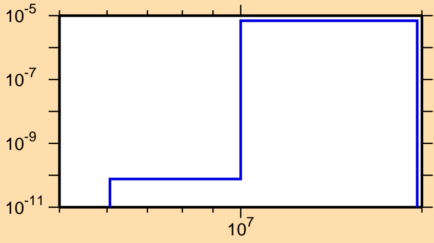
\sigma vs. E for ^{241}\text{Np}(n,n\alpha)
