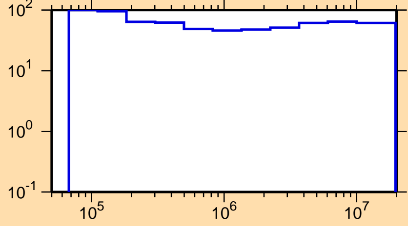
\Delta\sigma/\sigma vs. E for ^{241}\text{Np}(n,\text{inel.})
