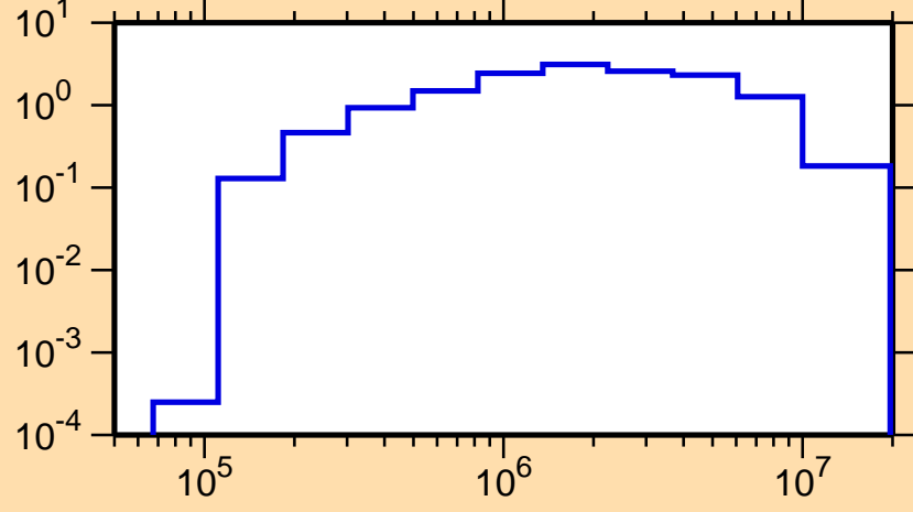
\sigma vs. E for ^{241}\text{Np}(n,\text{inel.})
