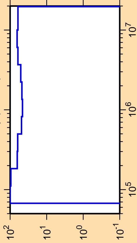
\Delta\sigma/\sigma vs. E for ^{241}\text{Np}(n,\text{inel.})
