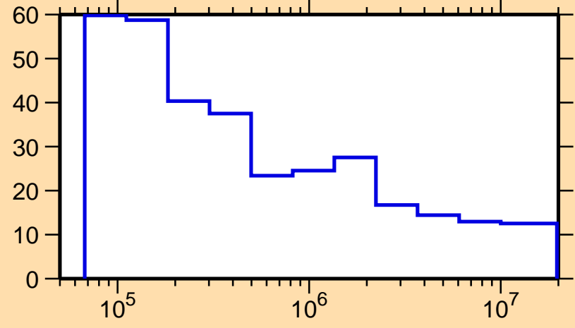
\Delta\sigma/\sigma vs. E for ^{241}\text{Np}(n,n\text{onel.})
