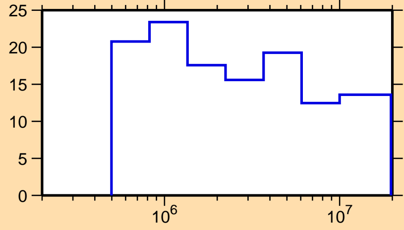
\Delta\sigma/\sigma vs. E for ^{242}\text{Np}(n,n\text{onel.})
