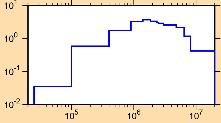
\sigma vs. E for ^{242}\text{Np}(n,\text{inel.})
