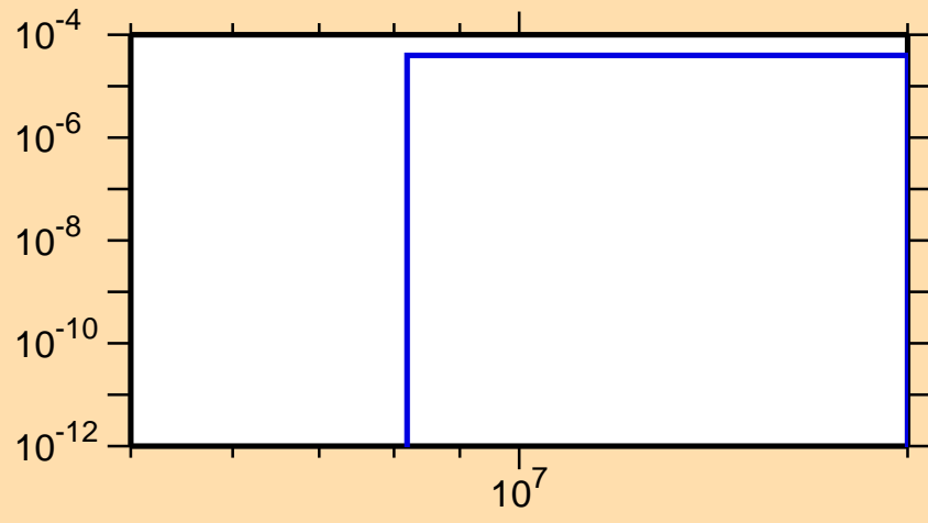
\sigma vs. E for ^{242}\text{Np}(n,t)
