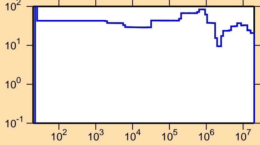
\Delta\sigma/\sigma vs. E for ^{242}\text{Np}(n,\text{el.})
