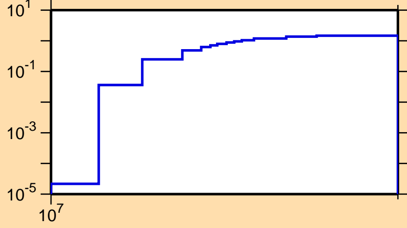
\sigma vs. E for ^{242}\text{Np}(n,3n)
