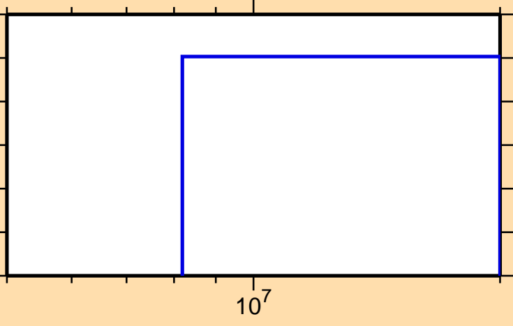
\sigma vs. E for ^{242}\text{Np}(n,\text{nd})
