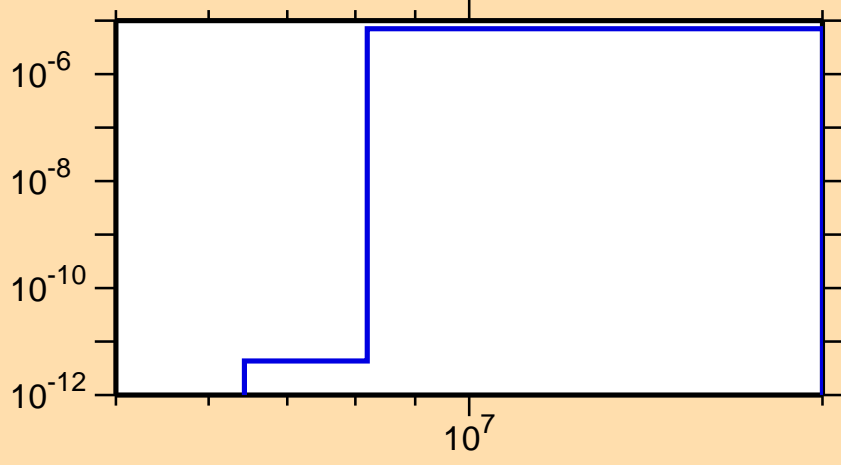
\sigma vs. E for ^{242}\text{Np}(n,\alpha)
