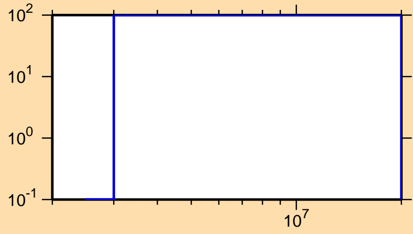
\Delta\sigma/\sigma vs. E for ^{242}\text{Np}(n,p)
