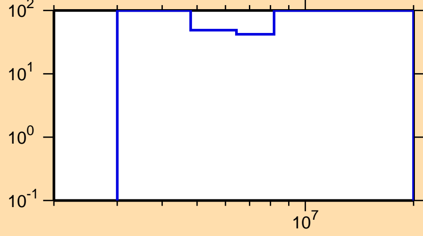
\Delta\sigma/\sigma vs. E for ^{242}\text{Np}(n,2n)
