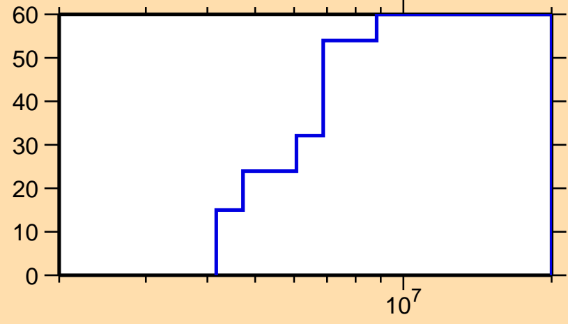
\Delta\sigma/\sigma vs. E for ^{243}\text{Np}(n,el.)
