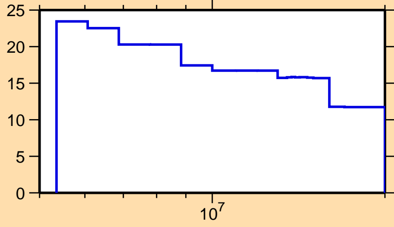
\Delta\sigma/\sigma vs. E for ^{243}\text{Np}(n,\text{nonel.})
