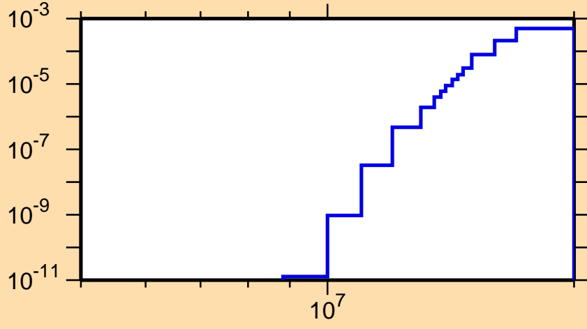
\sigma vs. E for ^{243}\text{Np}(n,t)
