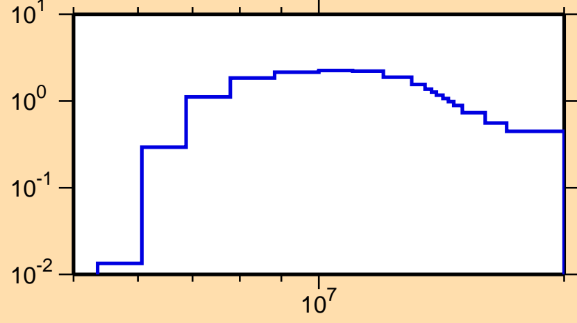
\sigma vs. E for ^{243}\text{Np}(n,2n)
