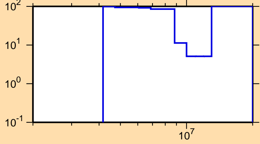
\Delta\sigma/\sigma vs. E for ^{243}\text{Np}(n,\gamma)
