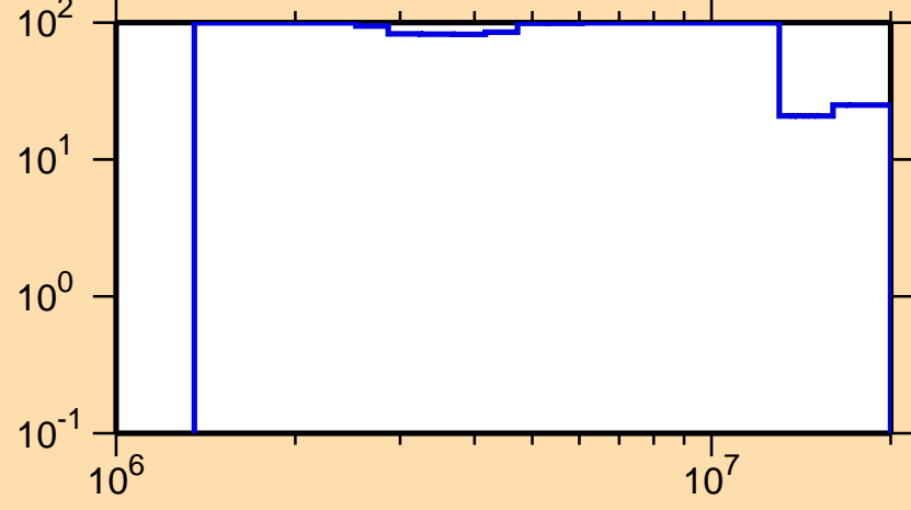
\Delta\sigma/\sigma vs. E for ^{243}\text{Np}(n,n\text{cont.})
