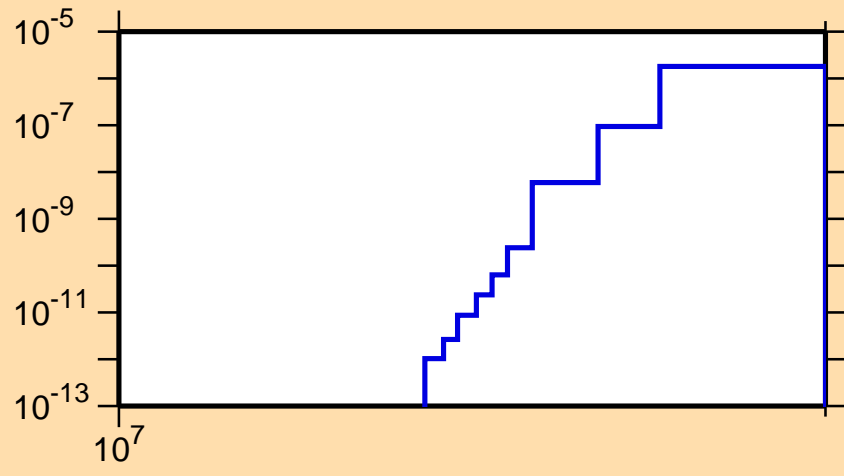
\sigma vs. E for ^{243}\text{Np}(n,\text{nd})
