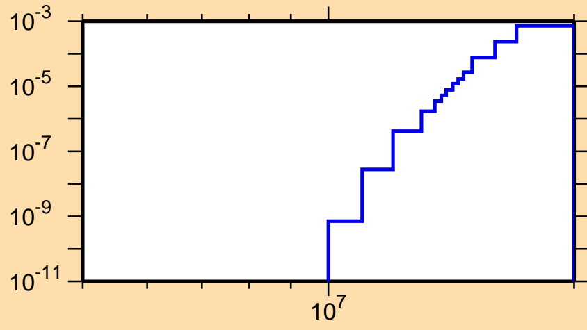
\sigma vs. E for ^{243}\text{Np}(n,np)
