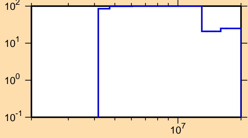
\Delta\sigma/\sigma vs. E for ^{243}\text{Np}(n,ncont.)
