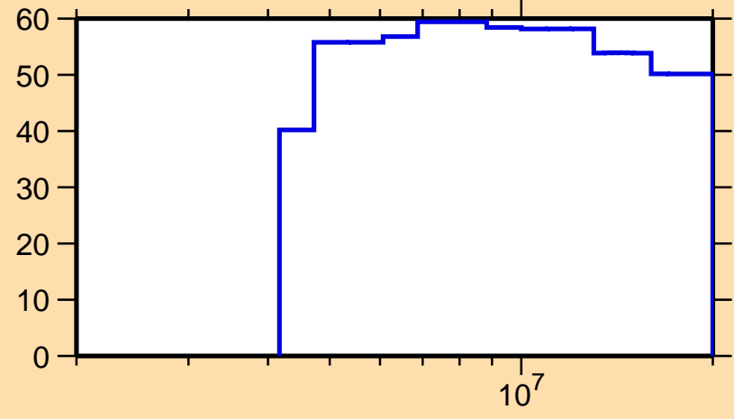
\Delta\sigma/\sigma vs. E for ^{243}\text{Np}(n,n_1)
