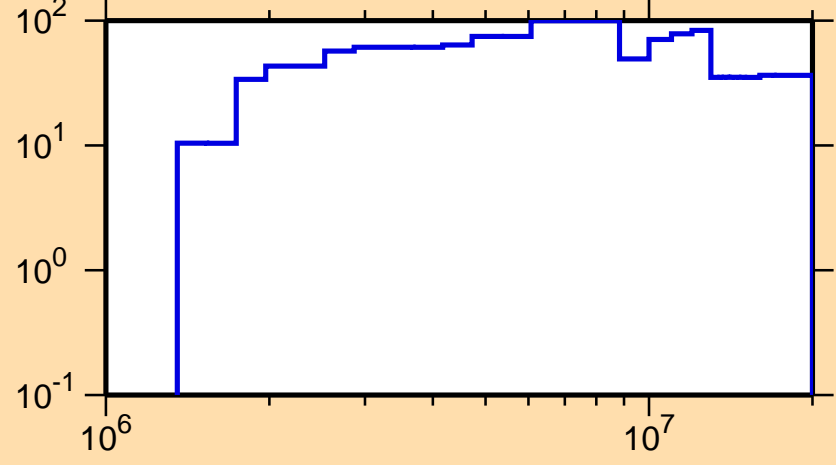
\Delta\sigma/\sigma vs. E for ^{243}\text{Np}(n,\text{inel.})
