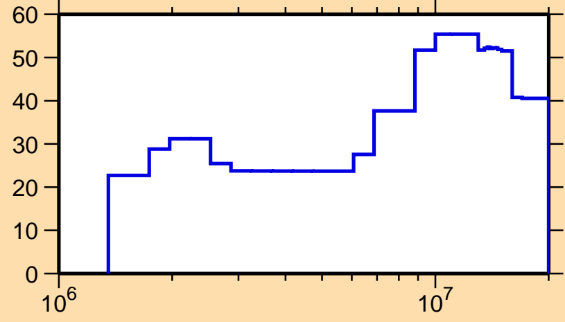
\Delta\sigma/\sigma vs. E for ^{243}\text{Np}(n,\text{tot.})
