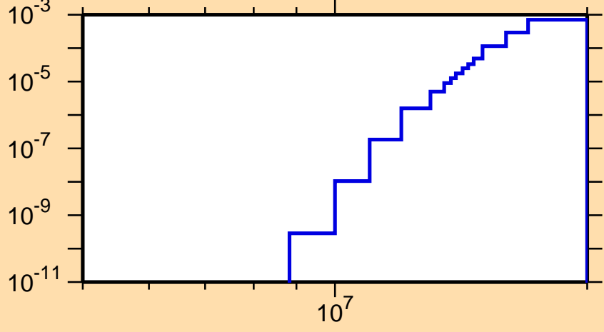
\sigma vs. E for ^{243}\text{Np}(n,d)
