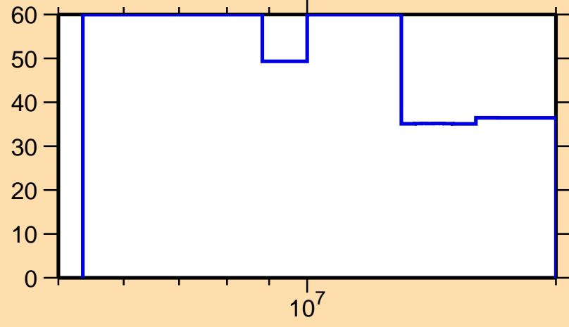
\Delta\sigma/\sigma vs. E for ^{243}\text{Np}(n,\text{inel.})
