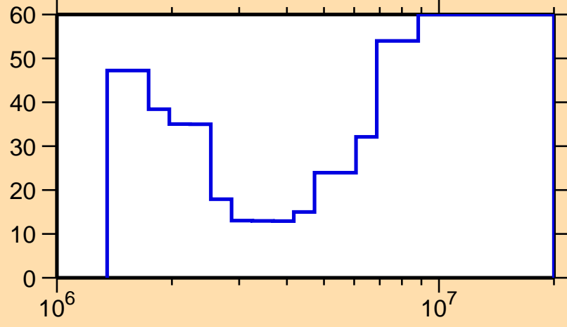
\Delta\sigma/\sigma vs. E for ^{243}\text{Np}(n,\text{el.})
