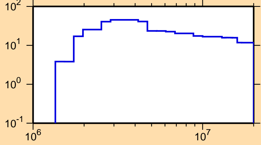
\Delta\sigma/\sigma vs. E for ^{243}\text{Np}(n,n\text{nonel.})
