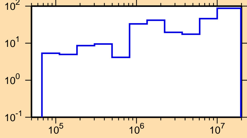
\Delta\sigma/\sigma vs. E for ^{243}\text{Np}(n,\text{el.})
