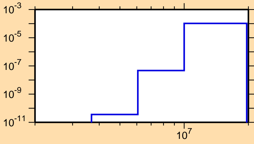
\sigma vs. E for ^{243}\text{Np}(n,\alpha)
