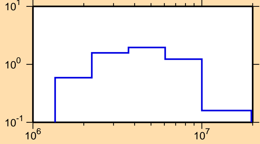
\sigma vs. E for ^{243}\text{Np}(n,n\text{cont.})
