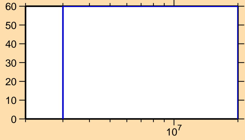
\Delta\sigma/\sigma vs. E for ^{243}\text{Np}(n,\gamma)
