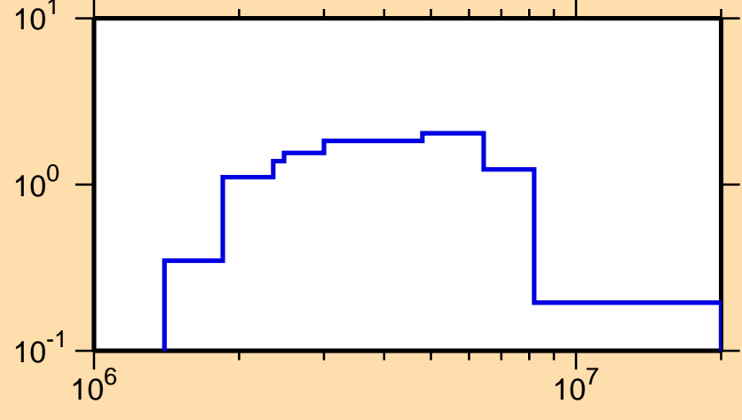
\sigma vs. E for ^{243}\text{Np}(n,n\text{cont.})
