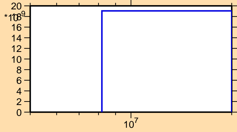
\sigma vs. E for ^{243}\text{Np}(n,\text{nd})
