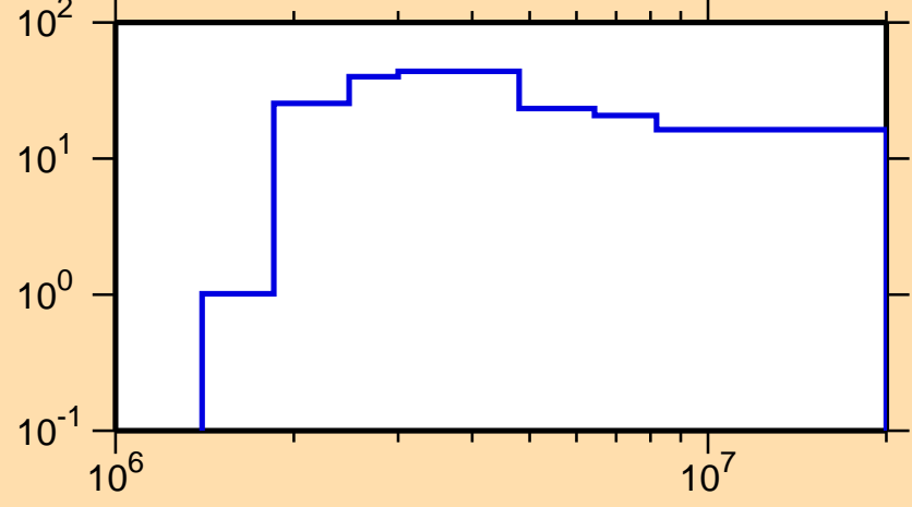
\Delta\sigma/\sigma vs. E for ^{243}\text{Np}(n,\text{nonel.})
