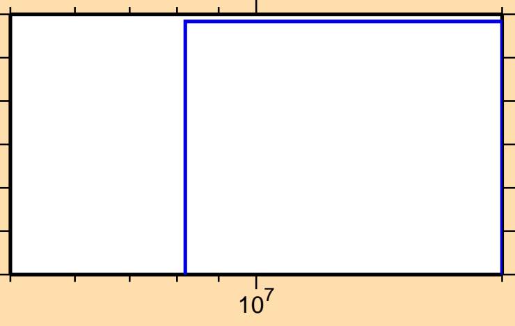
\sigma vs. E for ^{243}\text{Np}(n,np)
