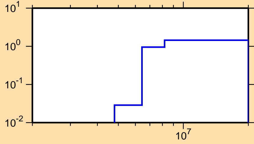
\sigma vs. E for ^{243}\text{Np}(n,2n)
