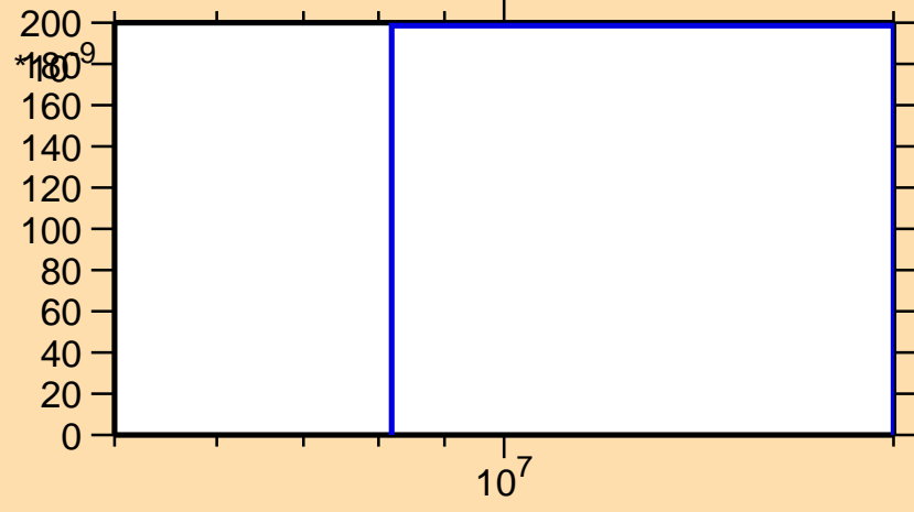
\sigma vs. E for ^{243}\text{Np}(n,nt)
