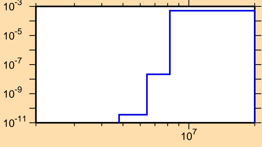
\sigma vs. E for ^{243}\text{Np}(n,p)
