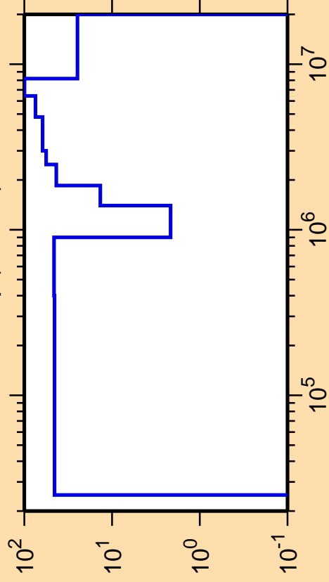
\Delta\sigma/\sigma vs. E for ^{243}\text{Np}(n,\text{inel.})
