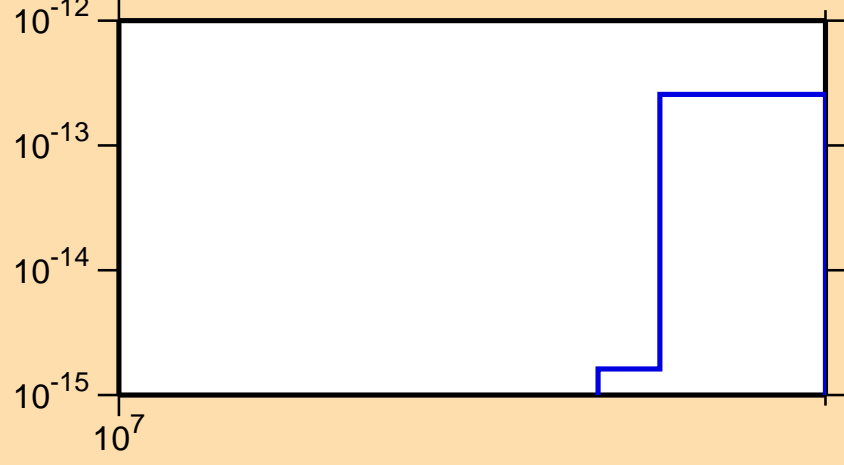
\sigma vs. E for ^{244}\text{Np}(n,\text{He3})
