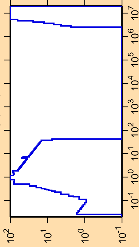
\Delta\sigma/\sigma vs. E for ^{244}\text{Np}(n,\alpha)
