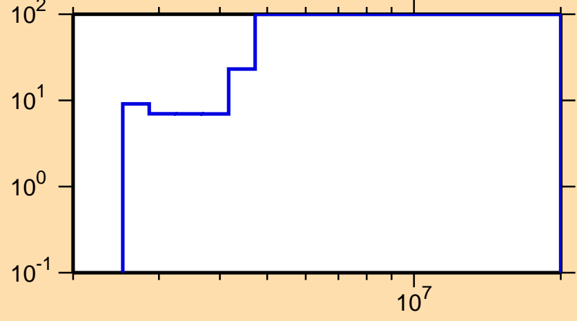
\Delta\sigma/\sigma vs. E for ^{244}\text{Np}(n,\text{inel.})
