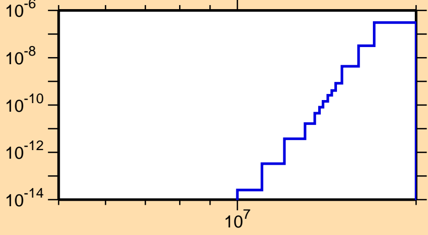
\sigma vs. E for ^{244}\text{Np}(n,2n\alpha)
