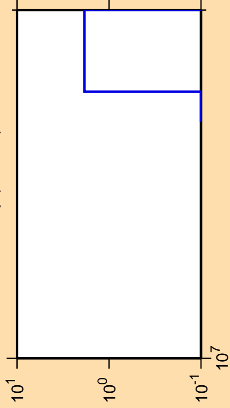
\Delta\sigma/\sigma vs. E for ^{244}\text{Np}(n,\text{He3})
