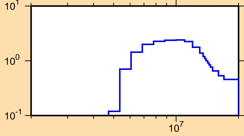
\sigma vs. E for ^{244}\text{Np}(n,2n)
