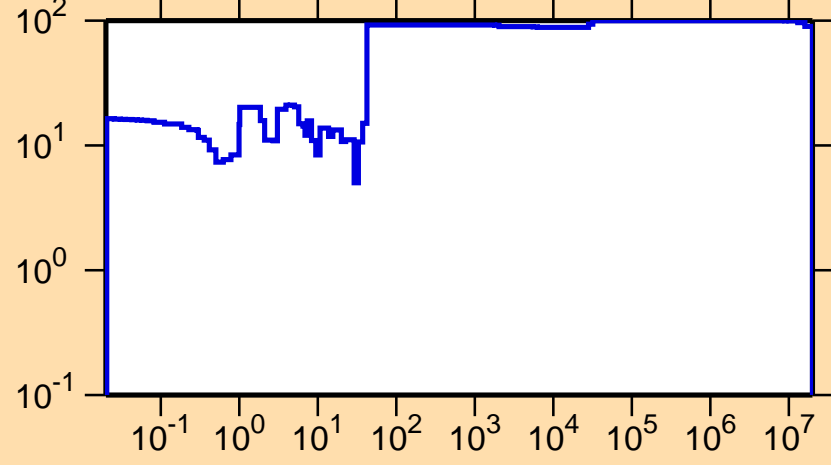
\Delta\sigma/\sigma vs. E for ^{244}\text{Np}(n,f)
