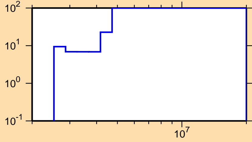
\Delta\sigma/\sigma vs. E for ^{244}\text{Np}(n,n\text{cont.})
