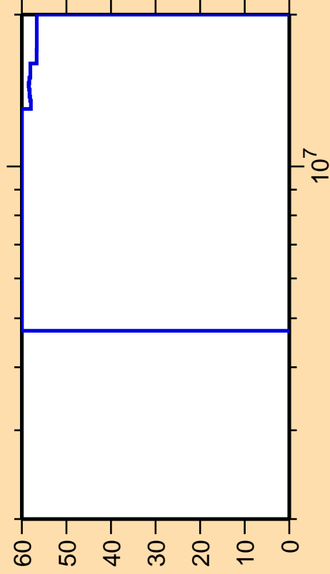
\Delta\sigma/\sigma vs. E for ^{244}\text{Np}(n,2n)
