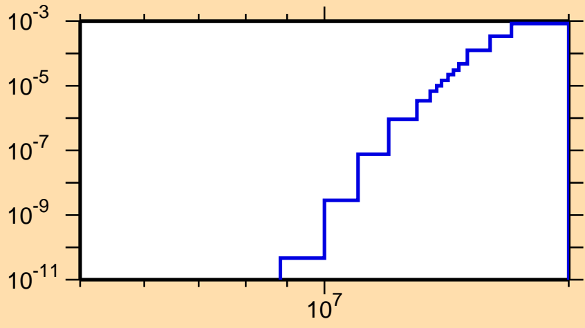
\sigma vs. E for ^{244}\text{Np}(n,d)
