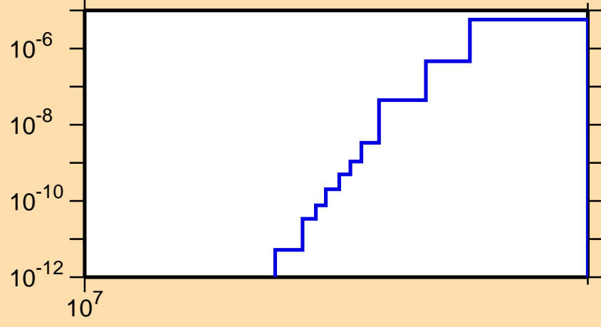
\sigma vs. E for ^{244}\text{Np}(n,\text{nd})
