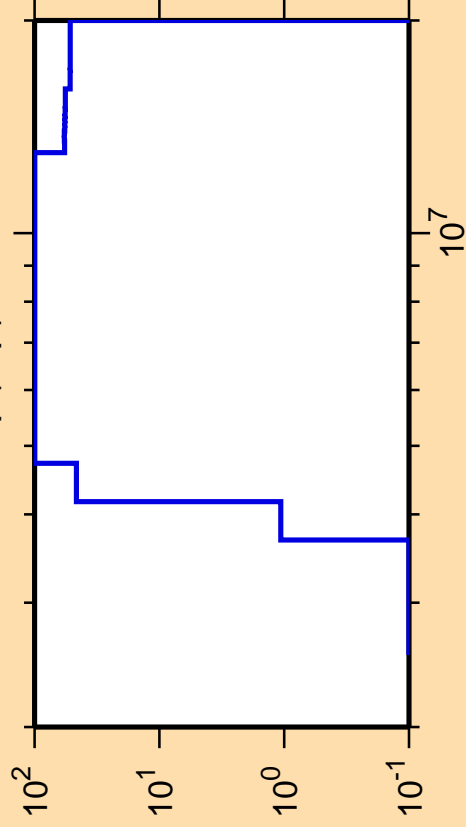
\Delta\sigma/\sigma vs. E for ^{244}\text{Np}(n,p)
