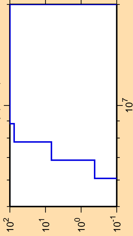
\Delta\sigma/\sigma vs. E for ^{244}\text{Np}(n,n\alpha)
