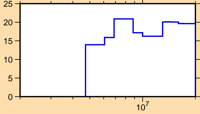
\Delta\sigma/\sigma vs. E for ^{244}\text{Np}(n,\text{nonel.})
