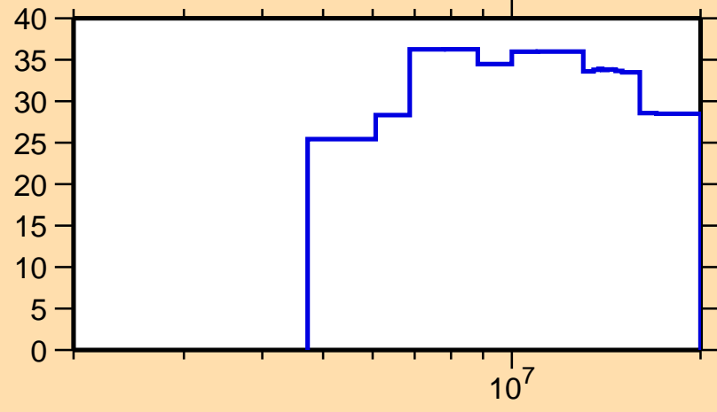
\Delta\sigma/\sigma vs. E for ^{244}\text{Np}(n,\text{el.})
