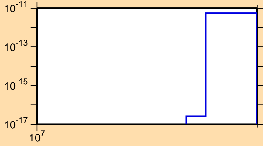
\sigma vs. E for ^{244}\text{Np}(\text{mt } 11)
