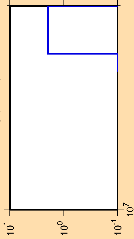
\Delta\sigma/\sigma vs. E for ^{244}\text{Np}(\text{mt } 11)
