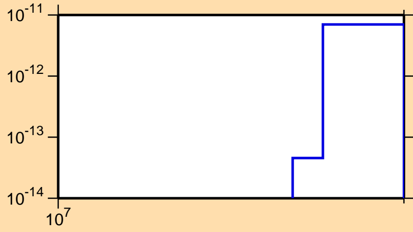
\sigma vs. E for ^{244}\text{Np}(n,3n\alpha)
