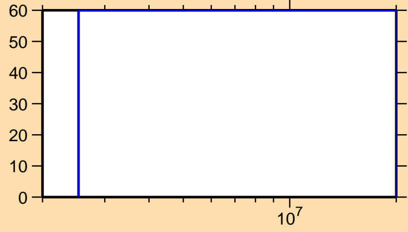
\Delta\sigma/\sigma vs. E for ^{244}\text{Np}(n,n_1)
