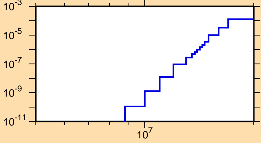
\sigma vs. E for ^{244}\text{Np}(n,n\alpha)
