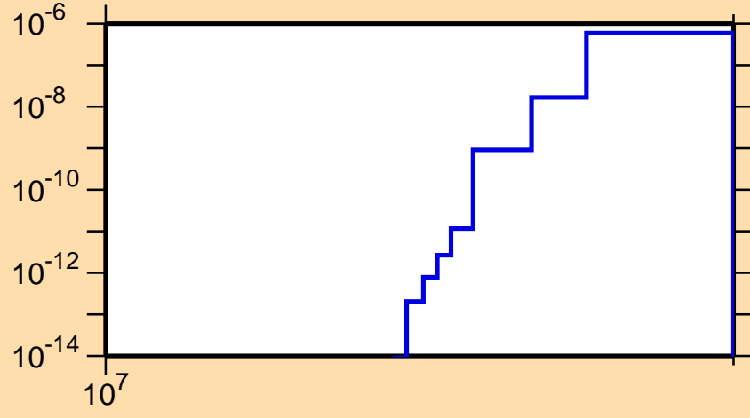
\sigma vs. E for ^{244}\text{Np}(n,2np)
