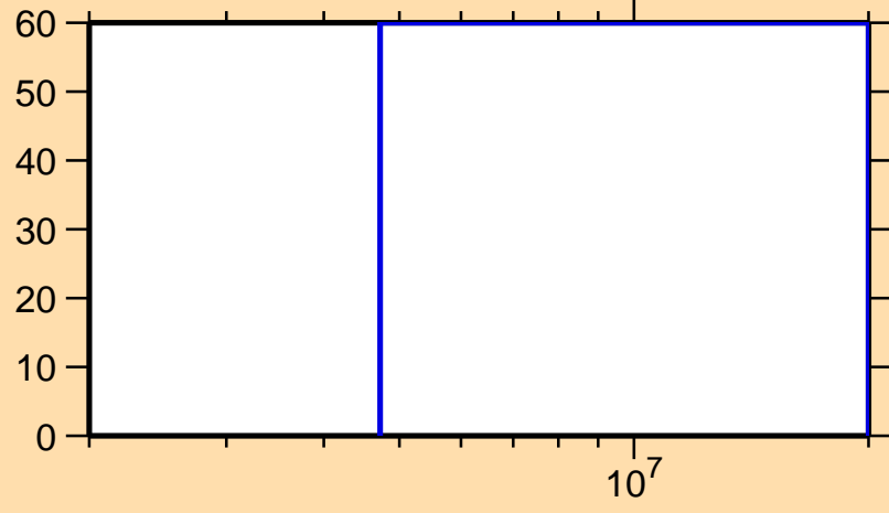
\Delta\sigma/\sigma vs. E for ^{244}\text{Np}(n,\text{inel.})
