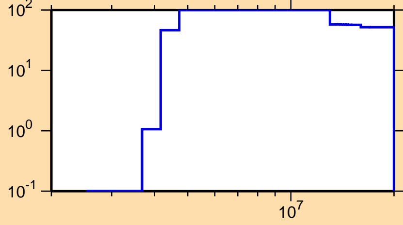
\Delta\sigma/\sigma vs. E for ^{244}\text{Np}(n,p)
