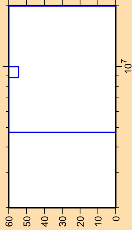
\Delta\sigma/\sigma vs. E for ^{244}\text{Np}(n,\gamma)
