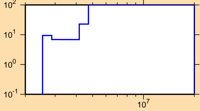
\Delta\sigma/\sigma vs. E for ^{244}\text{Np}(n,n\text{cont.})
