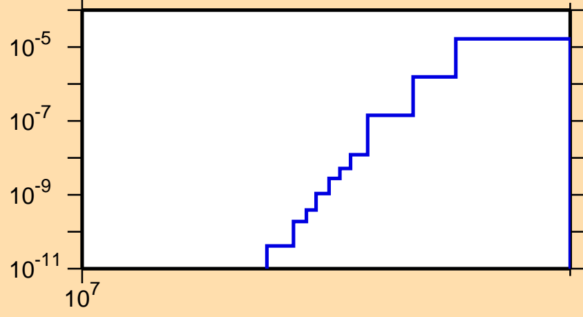
\sigma vs. E for ^{244}\text{Np}(n,nt)
