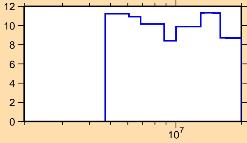
\Delta\sigma/\sigma vs. E for ^{244}\text{Np}(n,\text{tot.})
