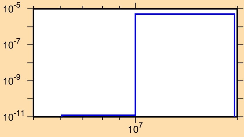
\sigma vs. E for ^{244}\text{Np}(n,n\alpha)
