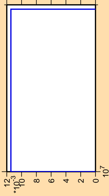
\Delta\sigma/\sigma vs. E for ^{244}\text{Np} (mt 11)
