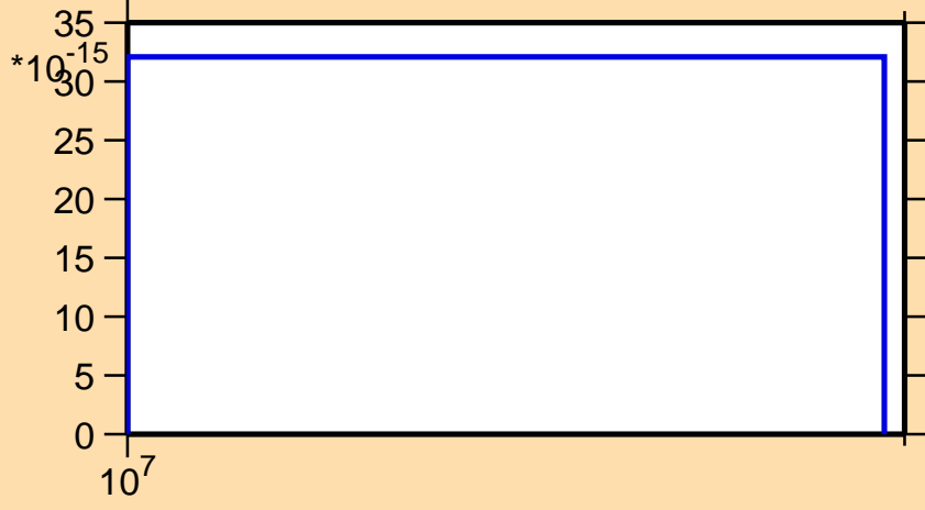
\sigma vs. E for ^{244}\text{Np} (mt 11)
