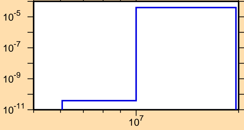
\sigma vs. E for ^{244}\text{Np}(n,t)
