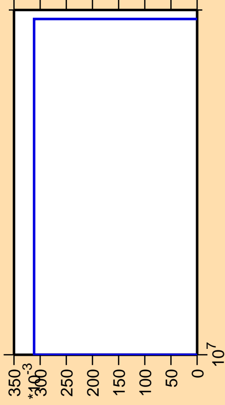
\Delta\sigma/\sigma vs. E for ^{244}\text{Np}(n,3n\alpha)
