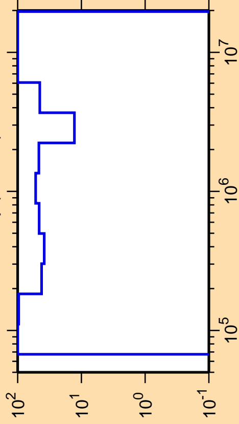
\Delta\sigma/\sigma vs. E for ^{244}\text{Np}(n,\text{inel.})
