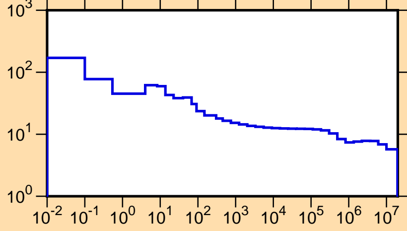
\sigma vs. E for ^{244}\text{Np}(n,\text{tot.})
