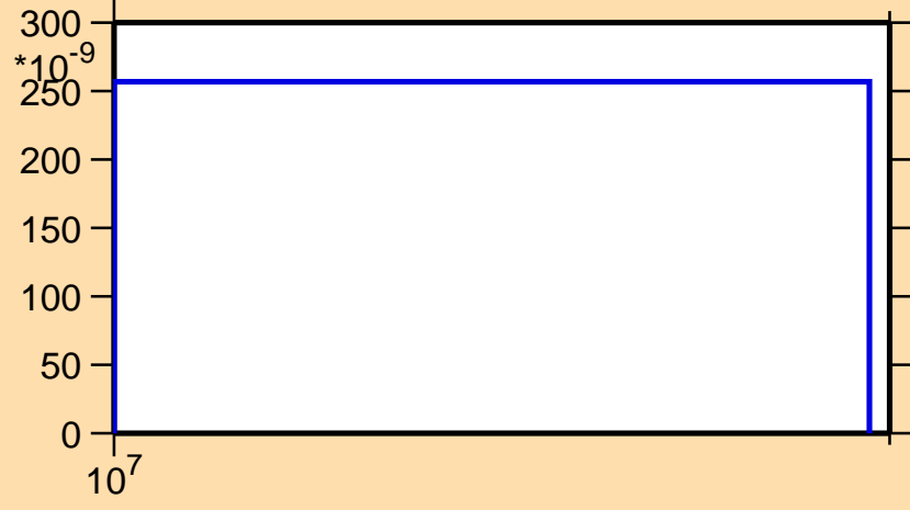
\sigma vs. E for ^{244}\text{Np}(n,nt)
