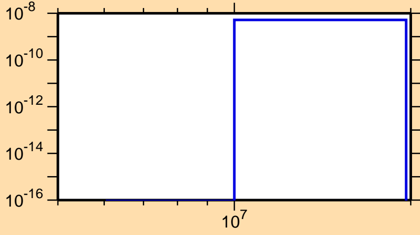
\sigma vs. E for ^{244}\text{Np}(n,2n\alpha)
