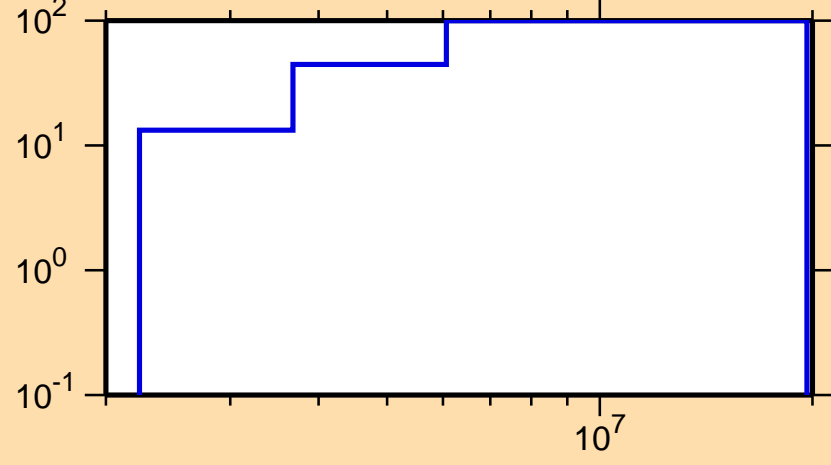
\Delta\sigma/\sigma vs. E for ^{244}\text{Np}(n,ncont.)
