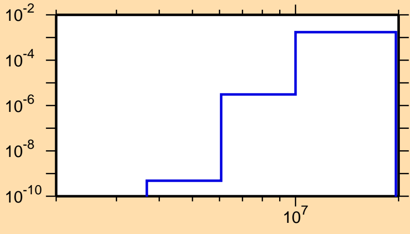
\sigma vs. E for ^{244}\text{Np}(n,p)
