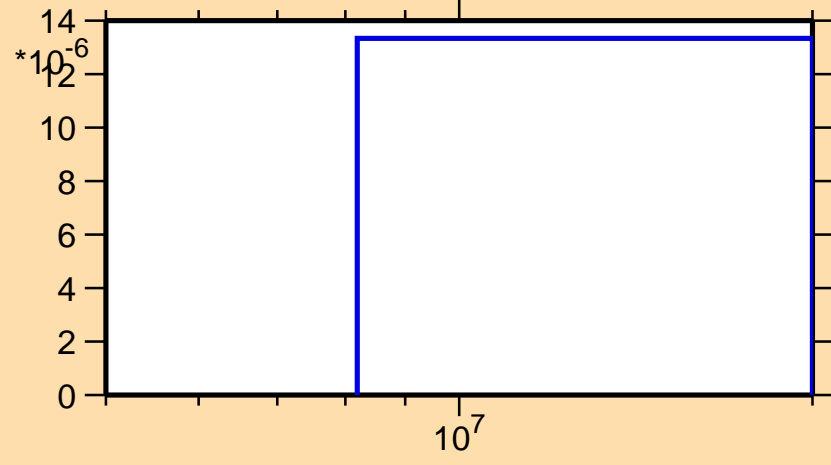
\sigma vs. E for ^{244}\text{Np}(n,np)
