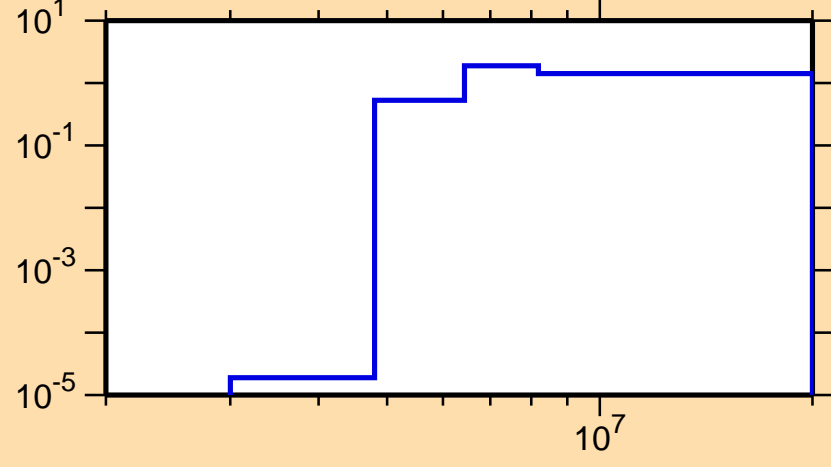
\sigma vs. E for ^{244}\text{Np}(n,2n)
