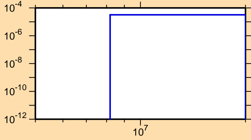
\sigma vs. E for ^{244}\text{Np}(n,t)
