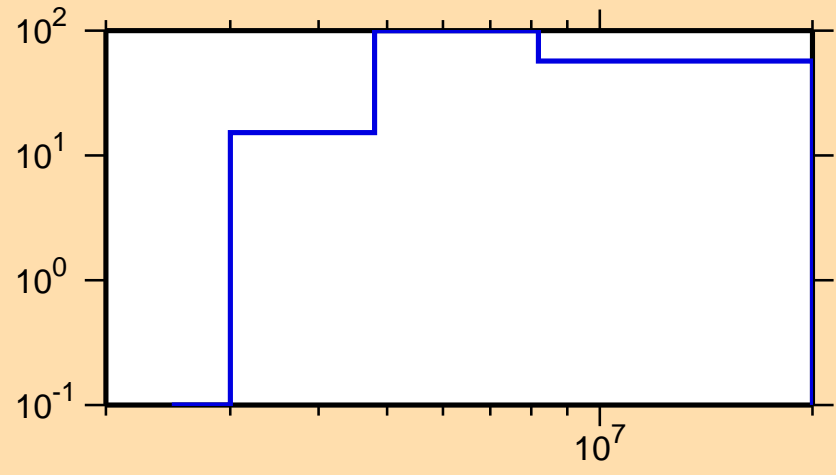
\Delta\sigma/\sigma vs. E for ^{244}\text{Np}(n,p)
