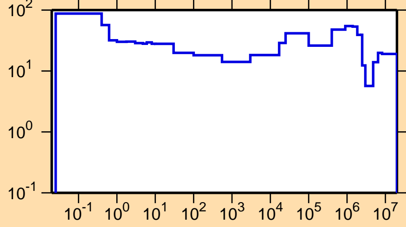
\Delta\sigma/\sigma vs. E for ^{244}\text{Np}(n,\text{nonel.})
