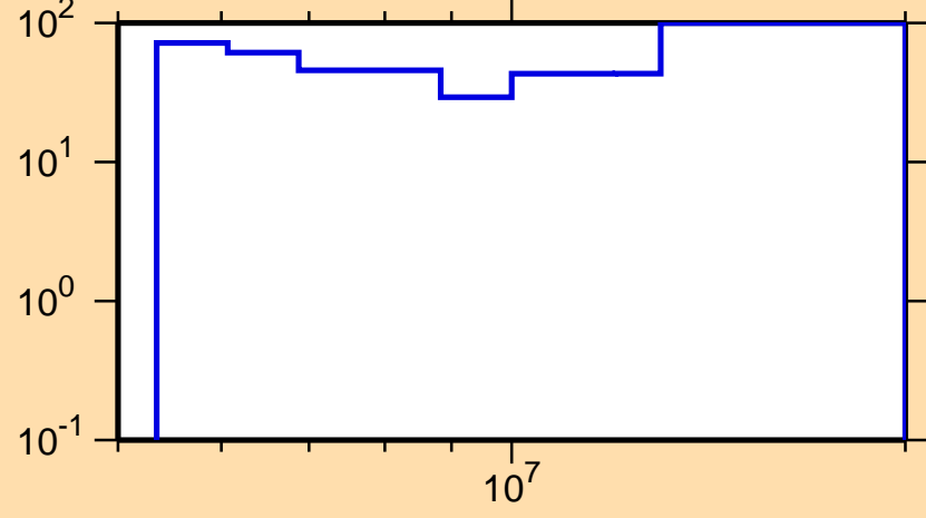
\Delta\sigma/\sigma vs. E for ^{245}\text{Np}(n,2n)
