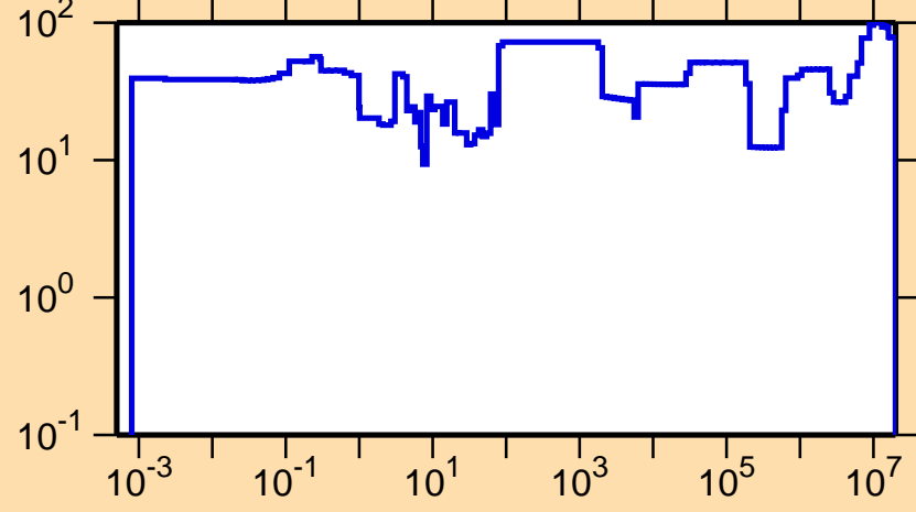
\Delta\sigma/\sigma vs. E for ^{245}\text{Np}(n,\text{tot.})
