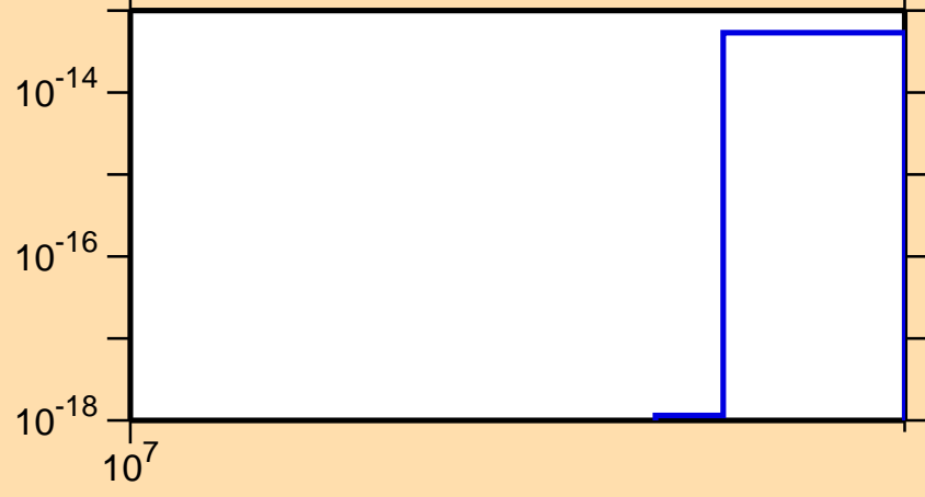
\sigma vs. E for ^{245}\text{Np}(n,\text{He3})
