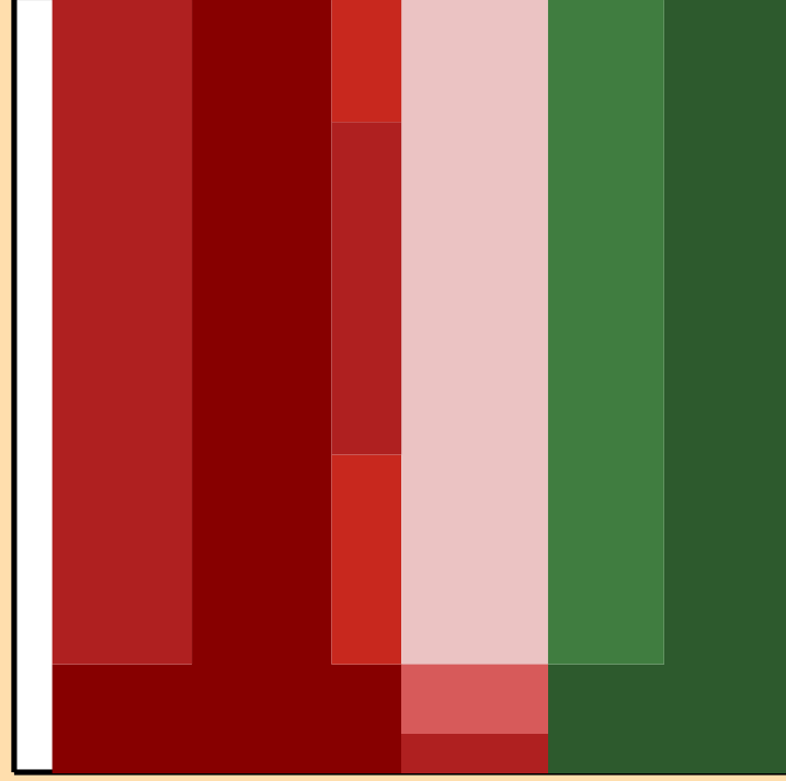
\Delta\sigma/\sigma vs. E for ^{245}\text{Np}(n,2n)
