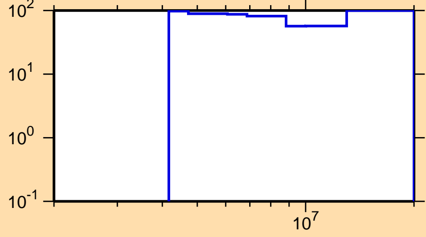
\Delta\sigma/\sigma vs. E for ^{245}\text{Np}(n,\gamma)
