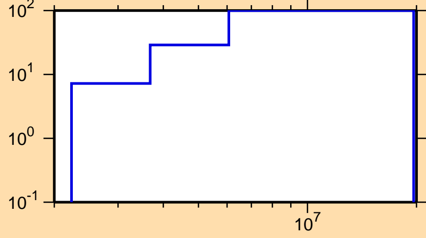
\Delta\sigma/\sigma vs. E for ^{245}\text{Np}(n,\text{inel.})
