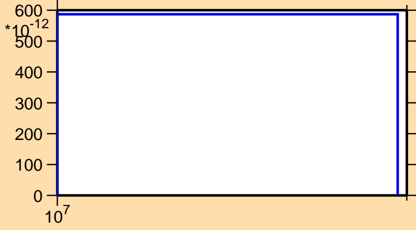
\sigma vs. E for ^{245}\text{Np}(n,2np)
