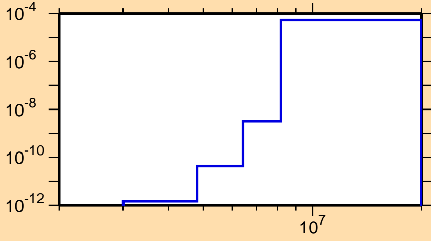
\sigma vs. E for ^{245}\text{Np}(n,\alpha)
