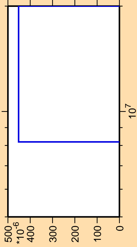
\Delta\sigma/\sigma vs. E for ^{245}\text{Np}(\text{mt } 42)
