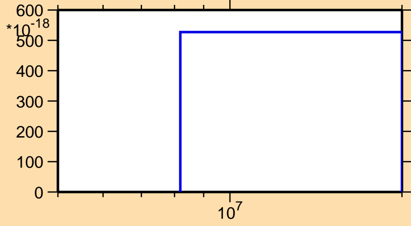
\sigma vs. E for ^{245}\text{Np}(\text{mt } 42)
