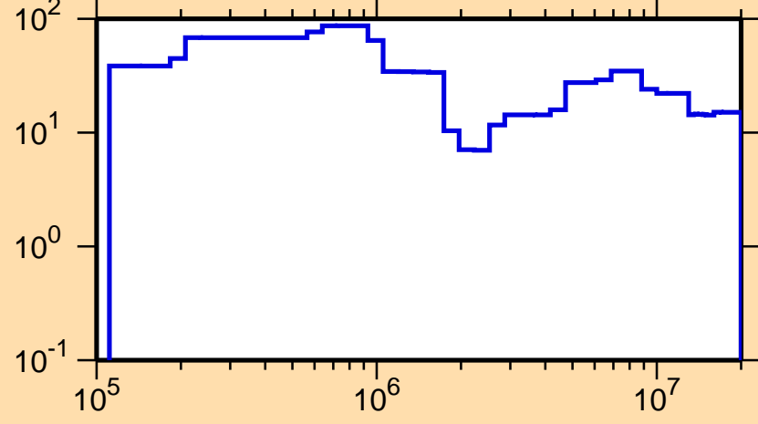
\Delta\sigma/\sigma vs. E for ^{225}\text{Pa}(n,\text{el.})
