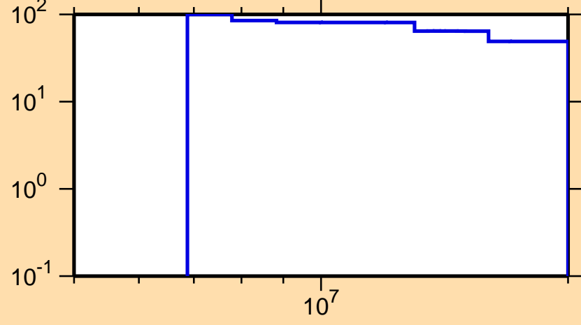
\Delta\sigma/\sigma vs. E for ^{225}\text{Pa}(n,2n)
