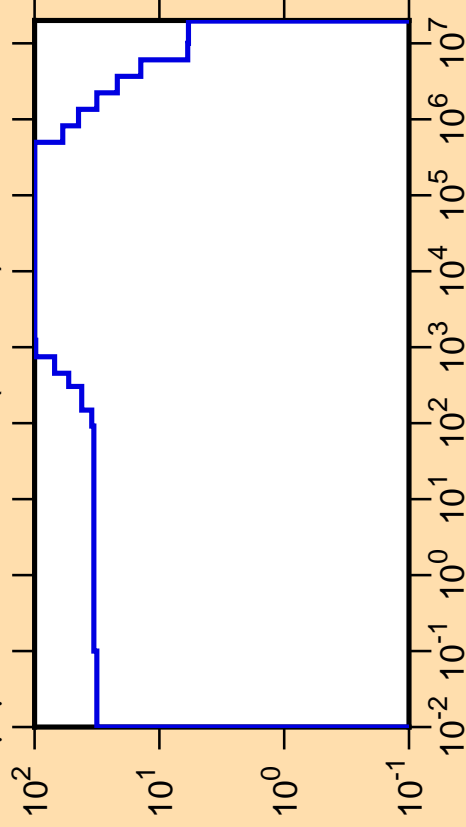
\Delta\mu/\mu vs. E for ^{225}\text{Pa}(\text{mt251})
