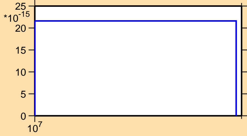
\sigma vs. E for ^{225}\text{Pa} (mt 34)
