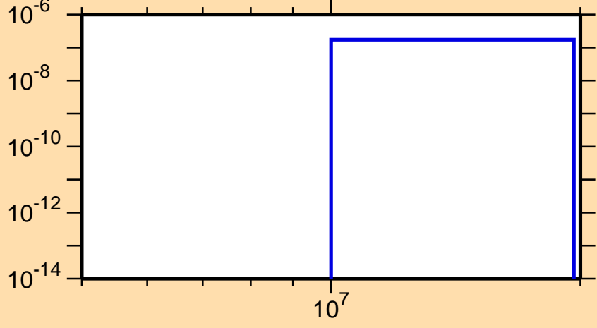
\sigma vs. E for ^{225}\text{Pa}(n,nt)
