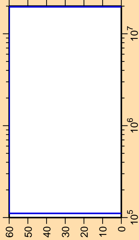
\Delta\sigma/\sigma vs. E for ^{225}\text{Pa}(n,\text{ncont.})
