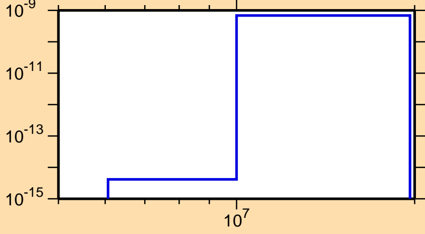
\sigma vs. E for ^{225}\text{Pa}(\text{mt117})
