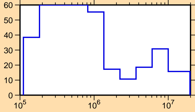
\Delta\sigma/\sigma vs. E for ^{225}\text{Pa}(n,\text{el.})
