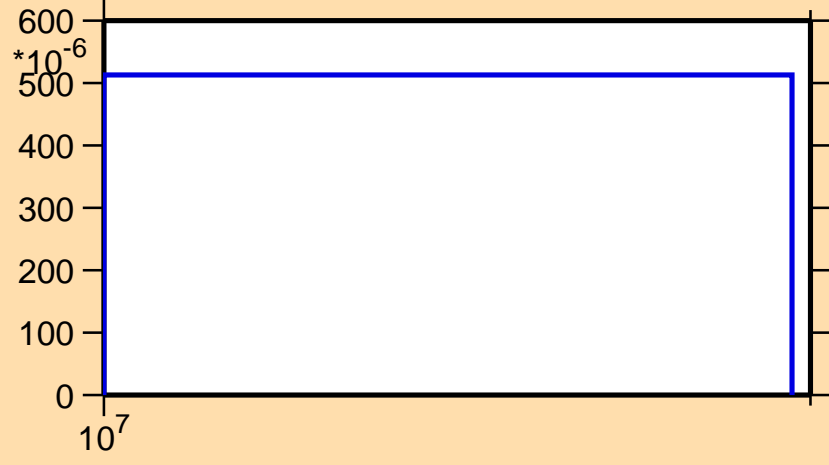
\sigma vs. E for ^{225}\text{Pa}(n,3n\alpha)
