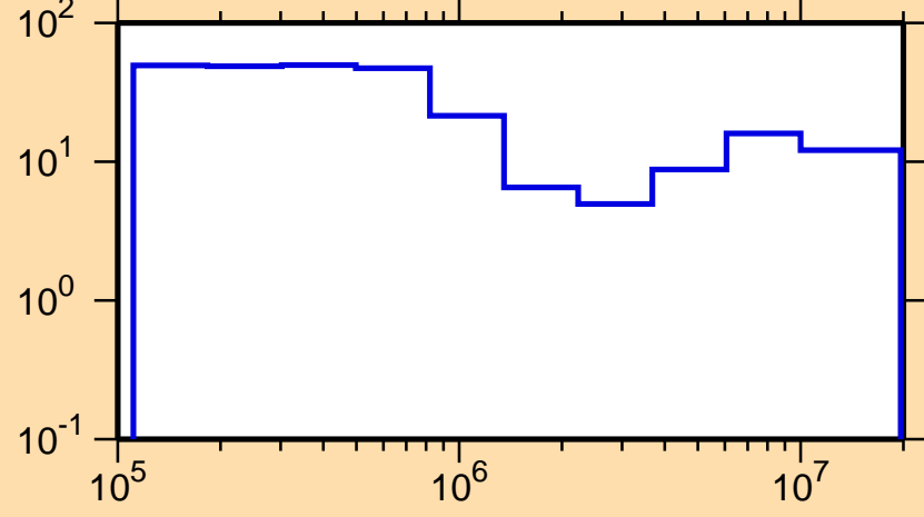
\Delta\sigma/\sigma vs. E for ^{225}\text{Pa}(n,\text{tot.})
