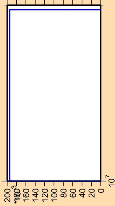
\Delta\sigma/\sigma vs. E for ^{225}\text{Pa} (mt 11)
