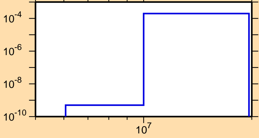
\sigma vs. E for ^{225}\text{Pa}(n,t)
