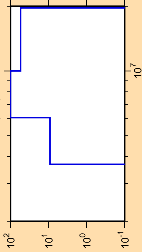
\Delta\sigma/\sigma vs. E for ^{225}\text{Pa}(n,d)
