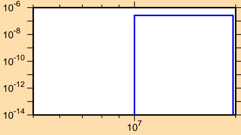
\sigma vs. E for ^{225}\text{Pa}(n,\text{nd})
