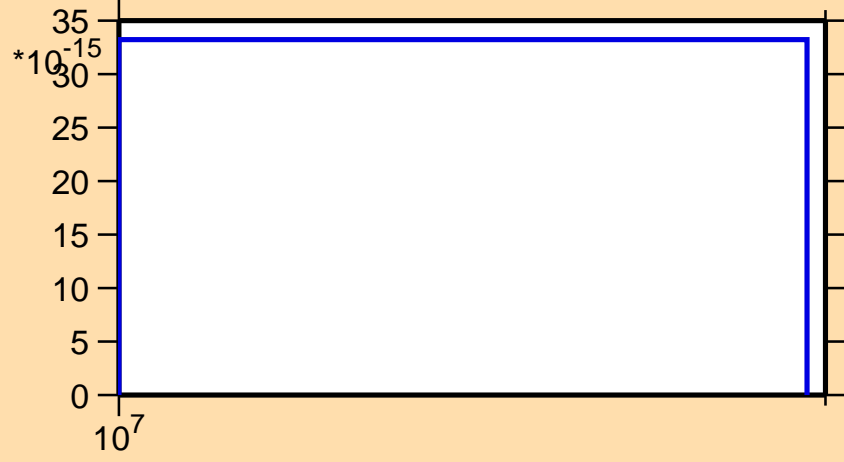
\sigma vs. E for ^{225}\text{Pa} (mt 11)
