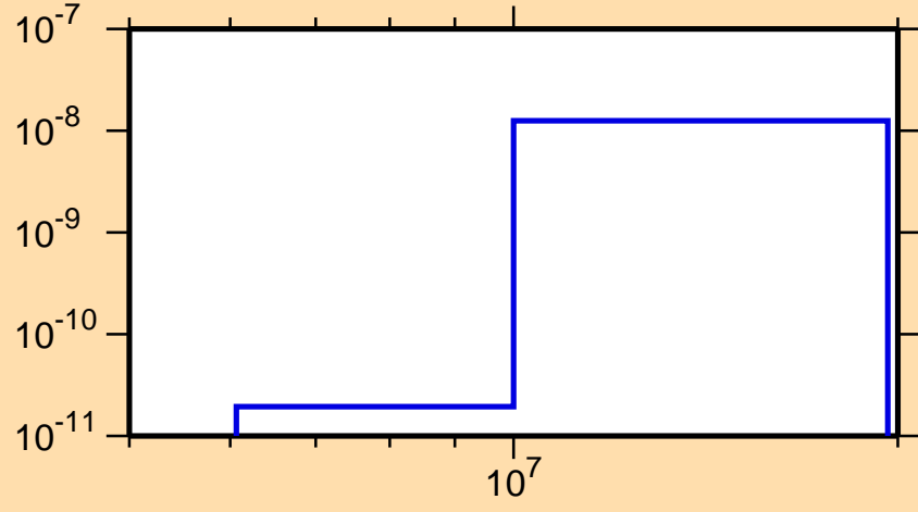
\sigma vs. E for ^{225}\text{Pa}(n,p\alpha)
