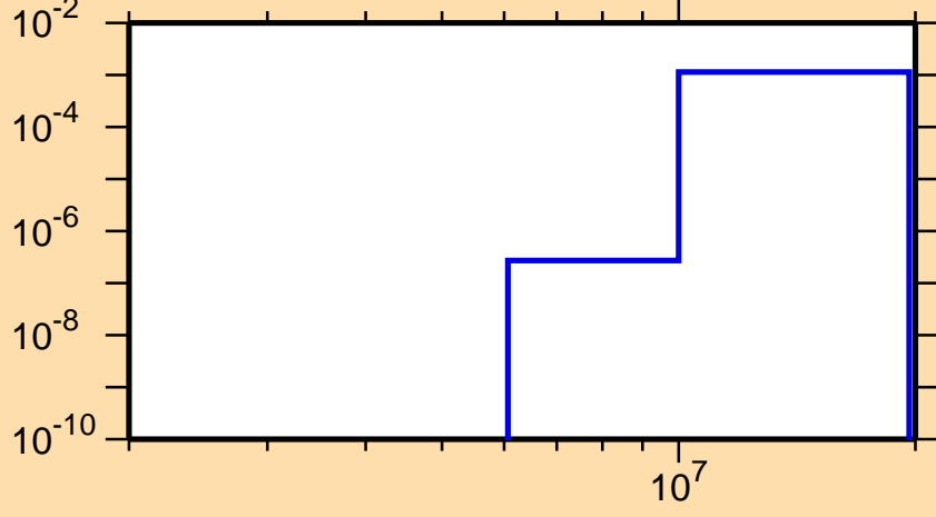
\sigma vs. E for ^{225}\text{Pa}(n,d)
