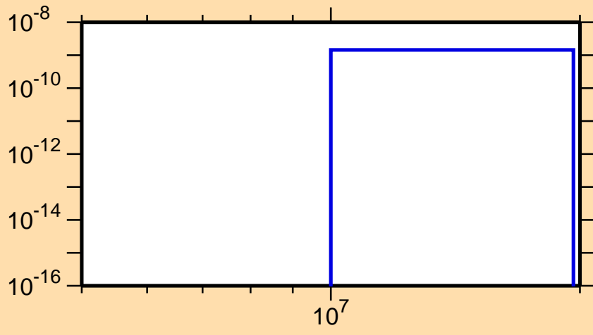
\sigma vs. E for ^{225}\text{Pa}(n,\text{He3})
