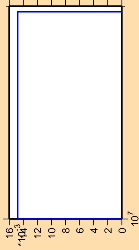
\Delta\sigma/\sigma vs. E for ^{225}\text{Pa} (mt 42)
