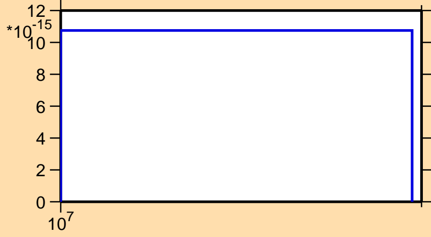
\sigma vs. E for ^{225}\text{Pa} (mt 42)
