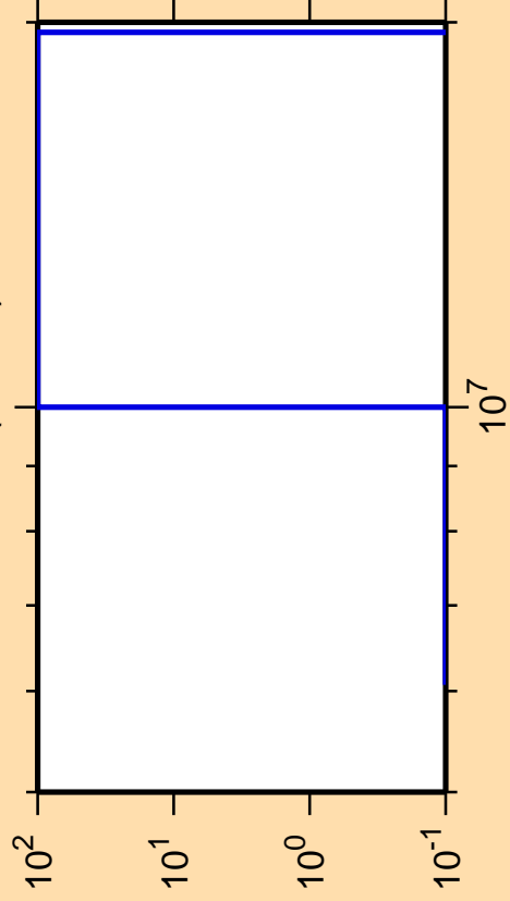
\Delta\sigma/\sigma vs. E for ^{225}\text{Pa}(\text{mt } 45)
