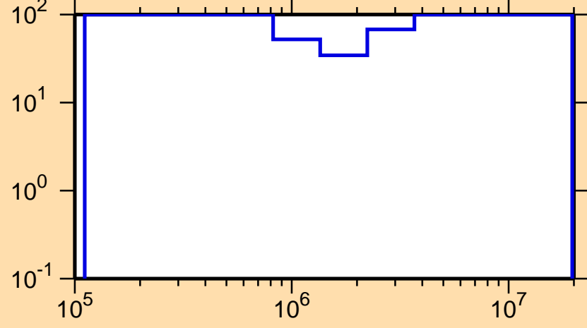
\Delta\sigma/\sigma vs. E for ^{225}\text{Pa}(n,f)
