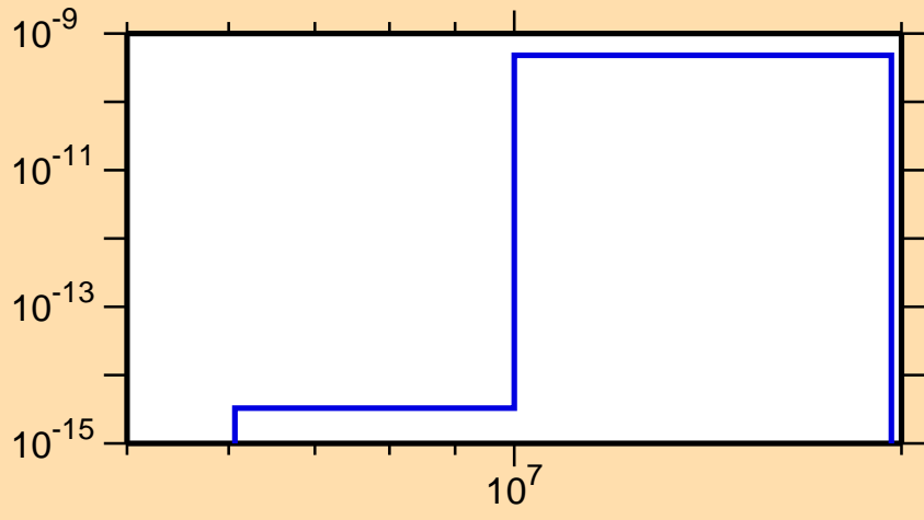
\sigma vs. E for ^{225}\text{Pa}(\text{mt } 45)
