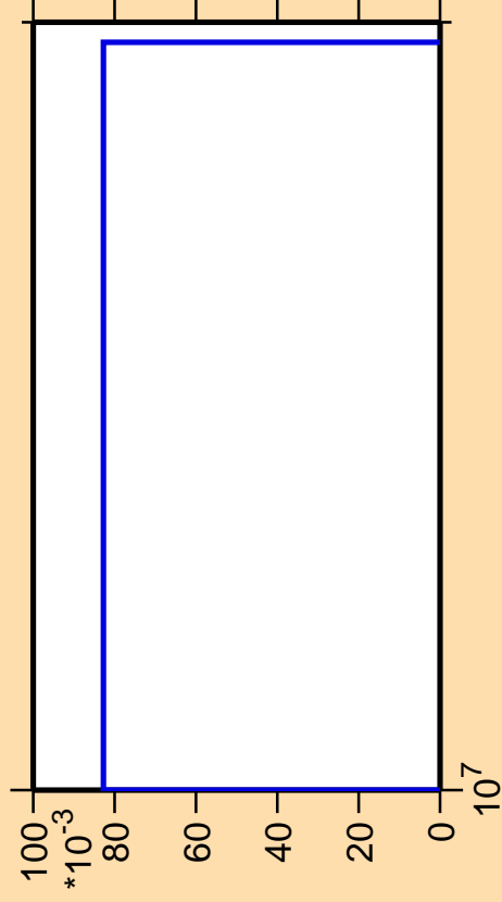
\Delta\sigma/\sigma vs. E for ^{225}\text{Pa} (mt 34)
