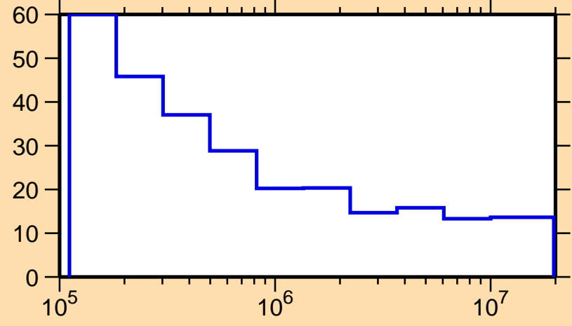
\Delta\sigma/\sigma vs. E for ^{225}\text{Pa}(n,\text{nonel.})
