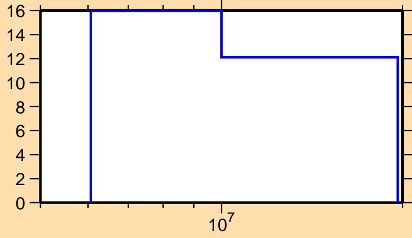
\Delta\sigma/\sigma vs. E for ^{225}\text{Pa}(n,\text{tot.})
